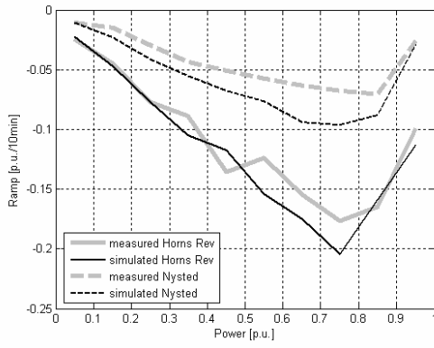
Figure 6. The 99% percentiles of 10-min ramp rates in all power ranges for Horns Rev and Nysted wind farm
