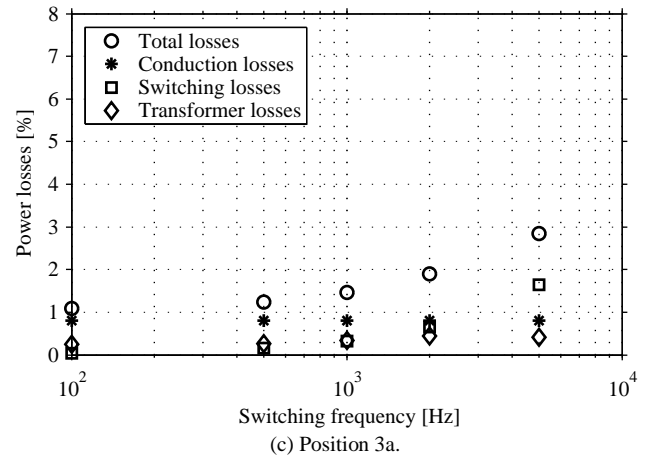
Figure 8. Loss distribution for IGBT module 2 using duty cycle control at the average wind speed 7.2m/s.
