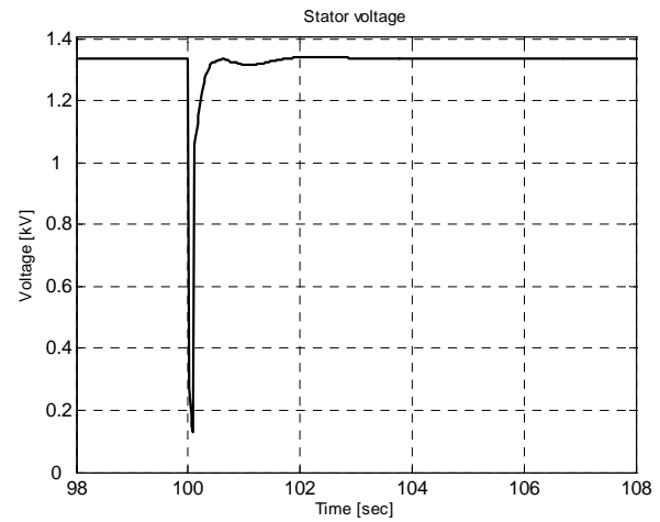
Figure 6. Generator stator voltage simulated DlgSILENT and used as input in HAWC2.
