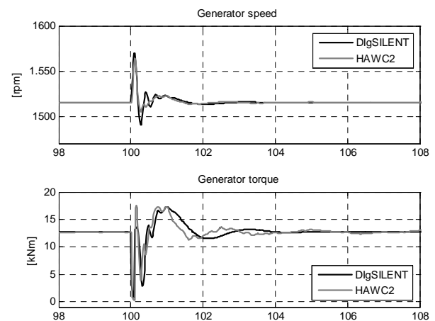
Figure 8. Generator speed and torque in DlgSILENT and HAWC2.
