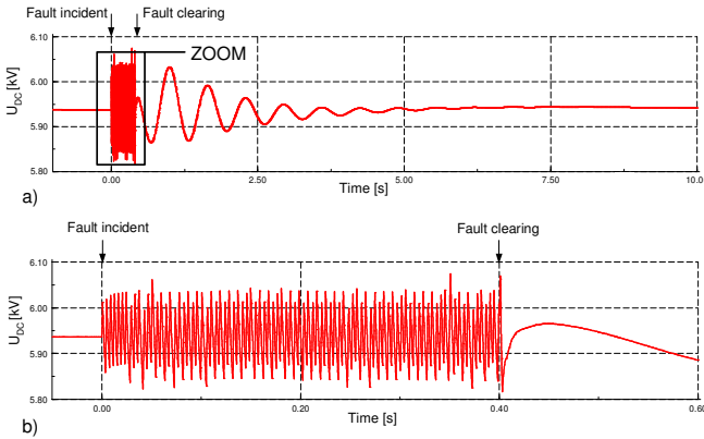
Figure 5: DC-voltage for a 400 ms three-phase fault at PMSG wind turbine's point of common coupling.
