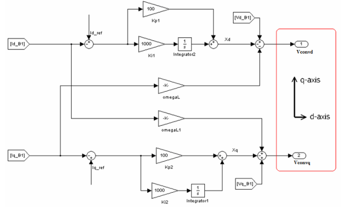
Figure 5 Current controller.
