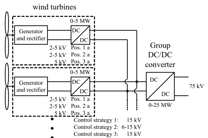
Figure 1. Local wind turbine grid with voltage levels.
