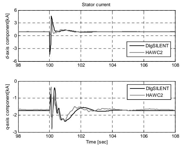
Figure 7. Components of the stator current on the d- and q- axis – simulated DlgSILENT and HAWC2.
