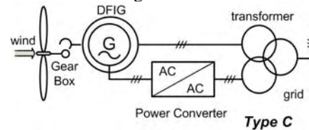
Figure 3. Variable speed wind turbine with partial scale power converter.
