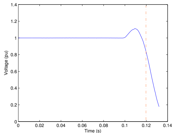
(b) Voltage space vector amplitude
