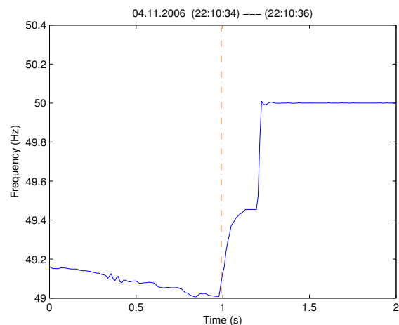
(c) Voltage frequency
