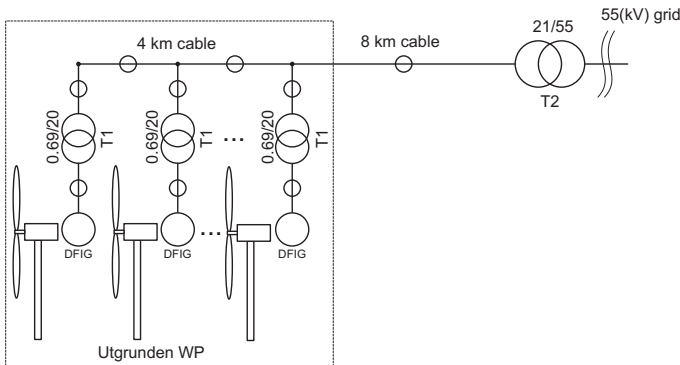
Fig. 1. Utgrunden WP, sea cable and 21/55 kV/kV substation
