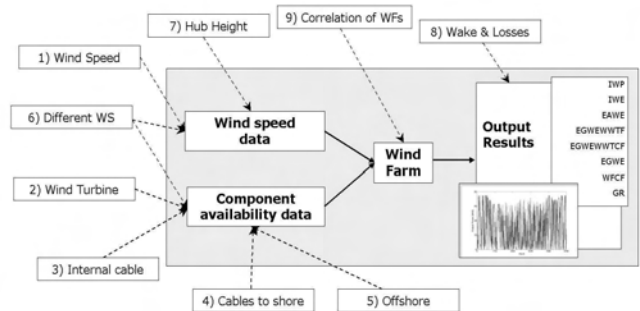
Figure 1. Wind farm reliability model: block diagram and influencing factors.
