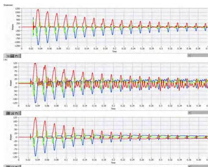
Figure 6 Current measurements at three locations during closing of the line breaker. Top: Transform platform, Middle: Turbine A01, Bottom: Turbine A09. Time: 20ms/div.
