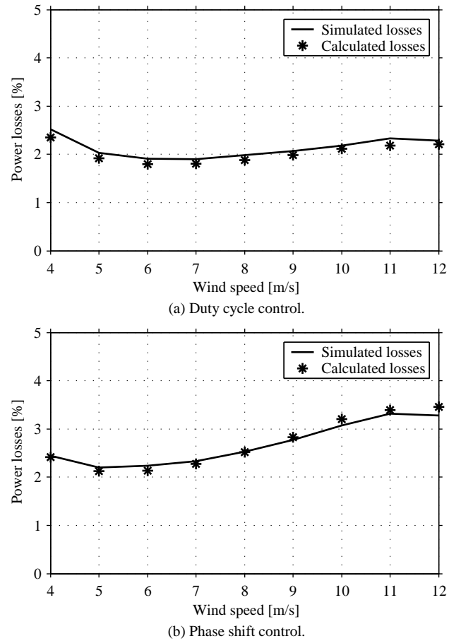
Figure 3. Resulting losses from calculations and simulations for position 1a.
