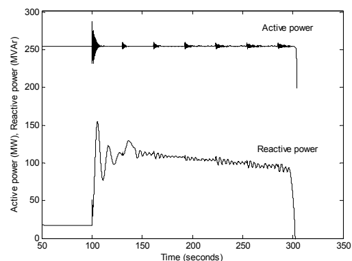
Figure 6. Synchronous generator active and reactive power.
