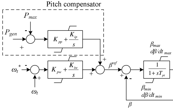
Fig. 9. Pitch controller
