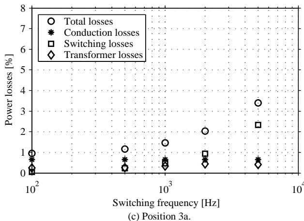
Figure 7. Loss distribution for IGBT module 1 using duty cycle control at the average wind speed 7.2 m/s.
