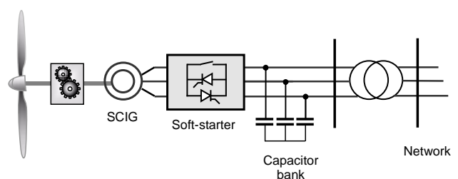
Figure 1. Schematic representation of a fixed-speed wind turbine
