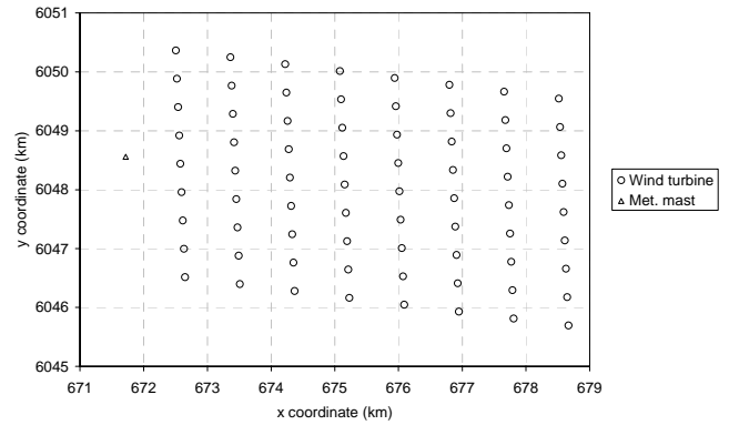
Figure 3. Nysted wind farm.
