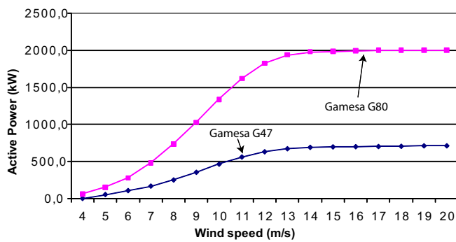
Fig. 2. Power curve of Gamesa G47 and G80
