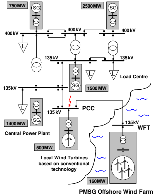
Figure 9: Generic power transmission system model
