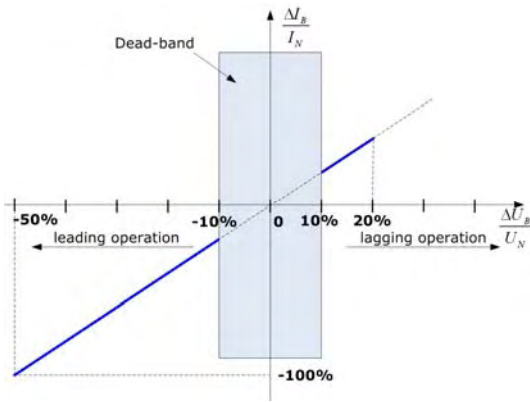
Figure 20. Grid support during faults by reactive current injection as specified in the German grid code for wind power [26], [27].
