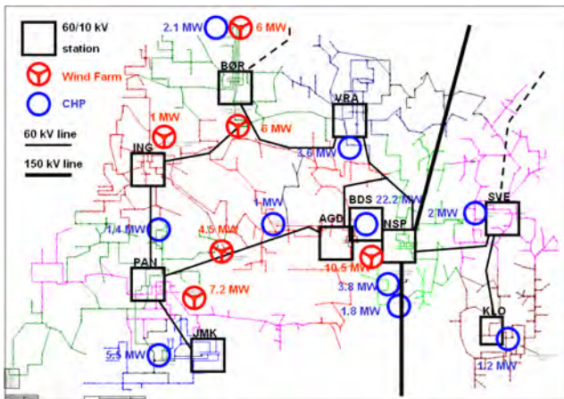
Fig. 1 The 60 and 10 kV network
