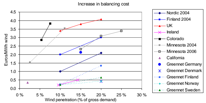
Figure 3. Results from estimates for the increase in balancing and operating costs due to wind power. The currency conversion used here is 1 \text{ €} = 0.7 \text{ £} and 1 \text{ €} = 1.3 \text{ US\$} .
