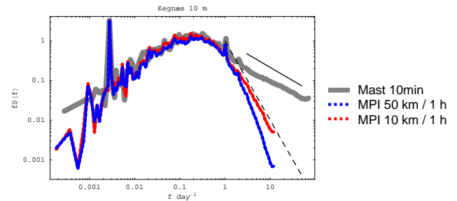
Figure 5. Measured (10m mast) PSD S_{[x,y]}(f) compared to climate model (MPI) PSD's S_{CM[x,y]}(f) for the Kegnæs site.
