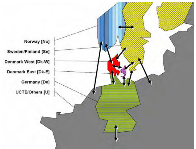
Figure 3. Price areas and their interconnections, as defined in the power market model. Copy from [5].
