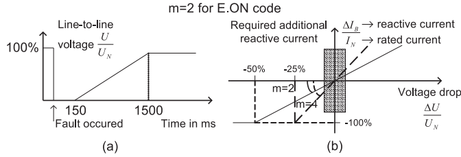
Fig. 1. The E.ON (a) voltage limit curve at the grid connection point during a fault and (b) the reactive power support required during a network fault.
