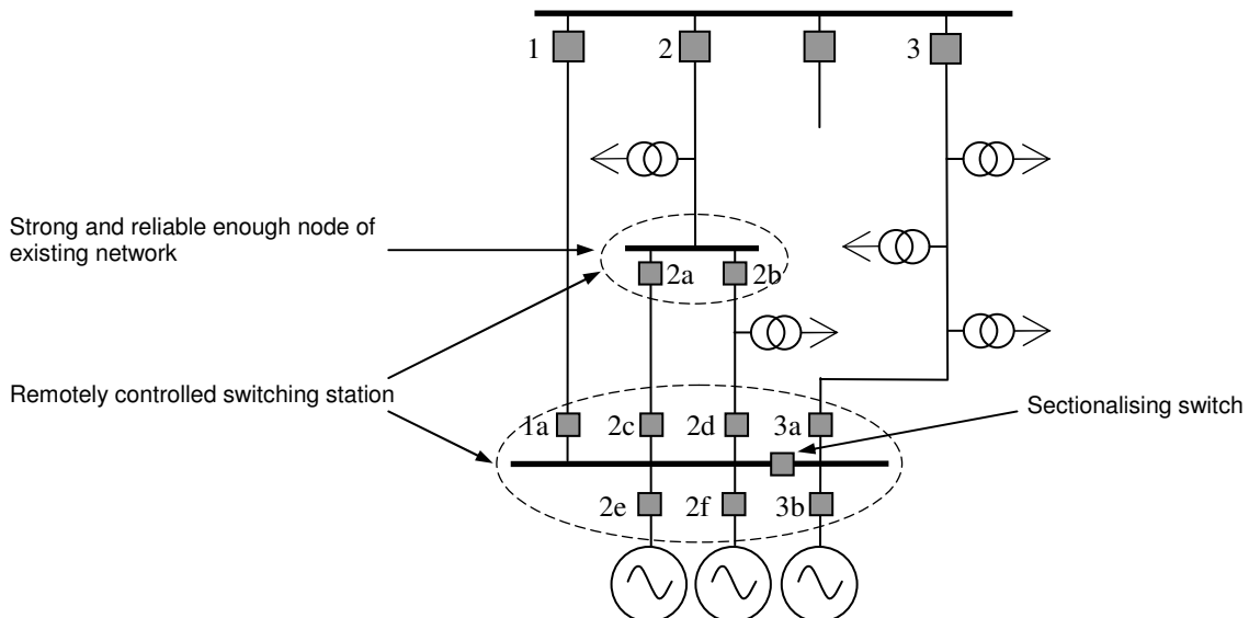
Figure 1. Possible network topologies.
