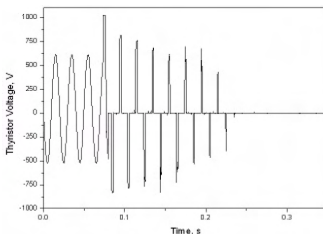
Figure 5. Instantaneous voltage across the thyristors (phase A) during the soft-start stage, recorded at Hagshaw Hill.
