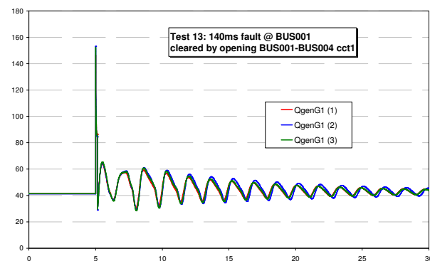
Figure 4: Reactive power of Test machine 1 in Test #13
