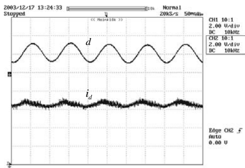
Figure 7. Waveforms of MPPT (E=160V)
