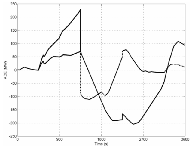
Fig. 6. ACE for the Dutch control zone with 4 GW wind power with perfect forecast d)(line) and with forecast errors e) (dotted line).
