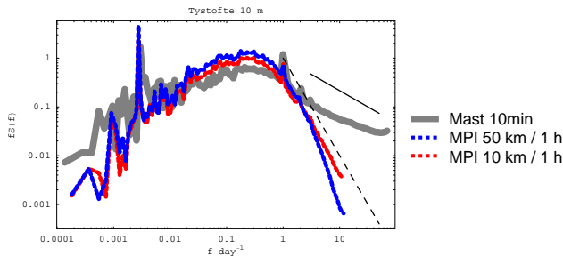
Figure 8. Measured (10m mast) PSD S_{[x,y]}(f) compared to climate model (MPI) PSD's S_{CM[x,y]}(f) for the Thystofte site.
