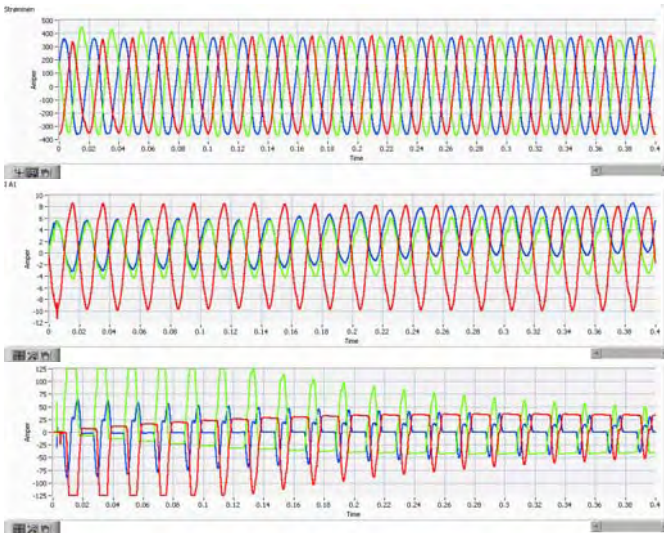
Figure 10 Current measurements at three locations during closing of switch in the wind turbine A09. Top: Transform platform, Middle: Turbine A01, Bottom: Turbine A09. Time: 20ms/div.
