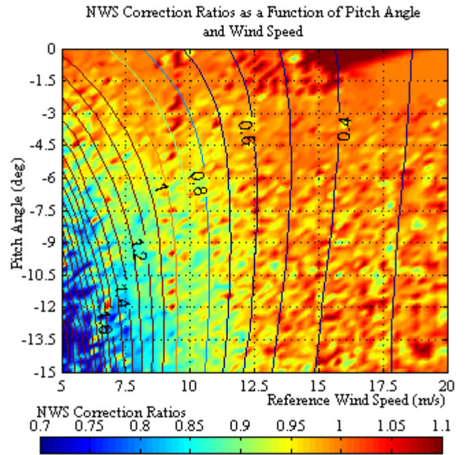
Figure 2-4: NWS correction Ratios as a Function of Pitch Angle and Wind Speed
