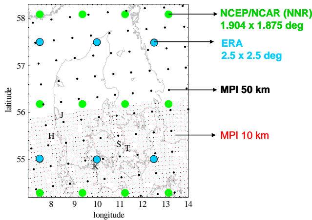
Figure 1. Climate models.
