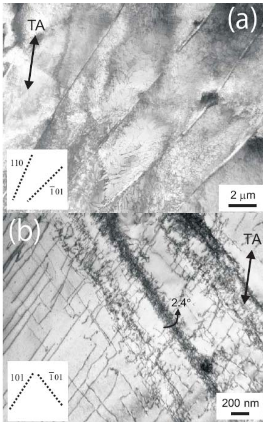
Figure 26. Microstructure in the Fe-Cr specimen post-irradiation tensile tested at 423 K. The specimen was irradiated (without any stress) at 327 K to a dose level of 6.5 \times 10^{-2} dpa prior to post-irradiation tensile test carried out with a strain rate of 1.3 \times 10^{-3} \text{ s}^{-1} . The microstructure illustrates the following: (a) formation of microbands extending over long distances ( >10 \mu\text{m} ) and (b) presence of long and straight dislocation lines and extended dense dislocation walls parallel to the (\bar{1}01) trace.
