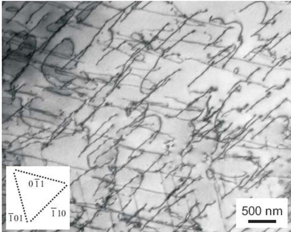
Figure 19. Dislocation microstructure in the Fe-Cr specimen (FC 20) used in the in-reactor Test No. 1 (see Figure 12 (a)) tensile tested at 325 K to a total strain level of 12.0 % (see Table 3) and to a dose level of 7.8 \times 10^{-2} dpa (see Table 2) with a strain rate of 1.0 \times 10^{-7} \text{ s}^{-1} showing relatively low density of mostly straight dislocations with a homogeneous distribution. Note that the straight dislocations are parallel to the traces of the three \{011\} planes (marked on the micrograph) lying in the [111] zone axis.
