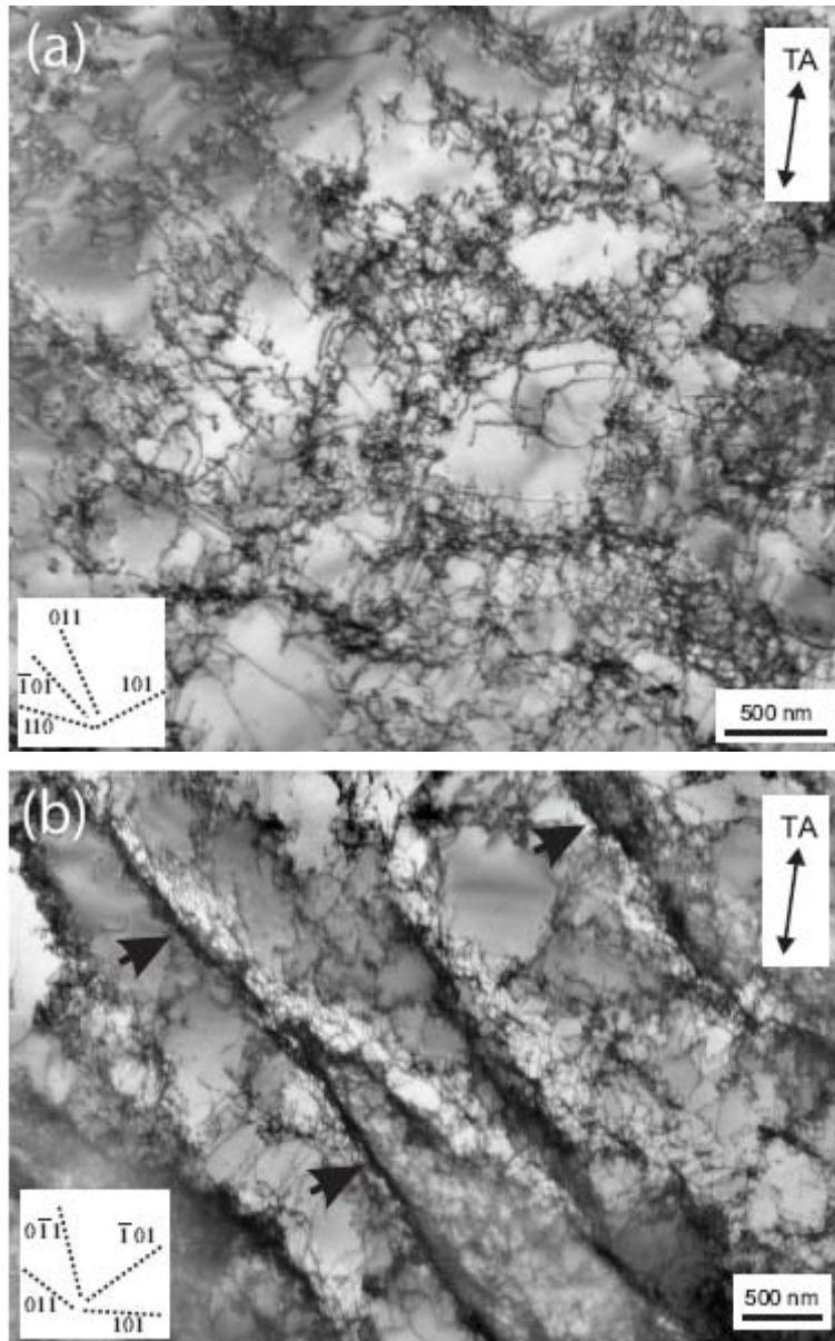
Figure 14. Same as in Figure 13 for Fe-Cr specimen tensile tested to a total strain level of 5 % showing (a) a typical cell structure with the cell boundaries of high dislocation density and the cell interiors almost free of dislocations and (b) long and dense dislocation walls (indicated by arrows) and loose cells between the walls.
