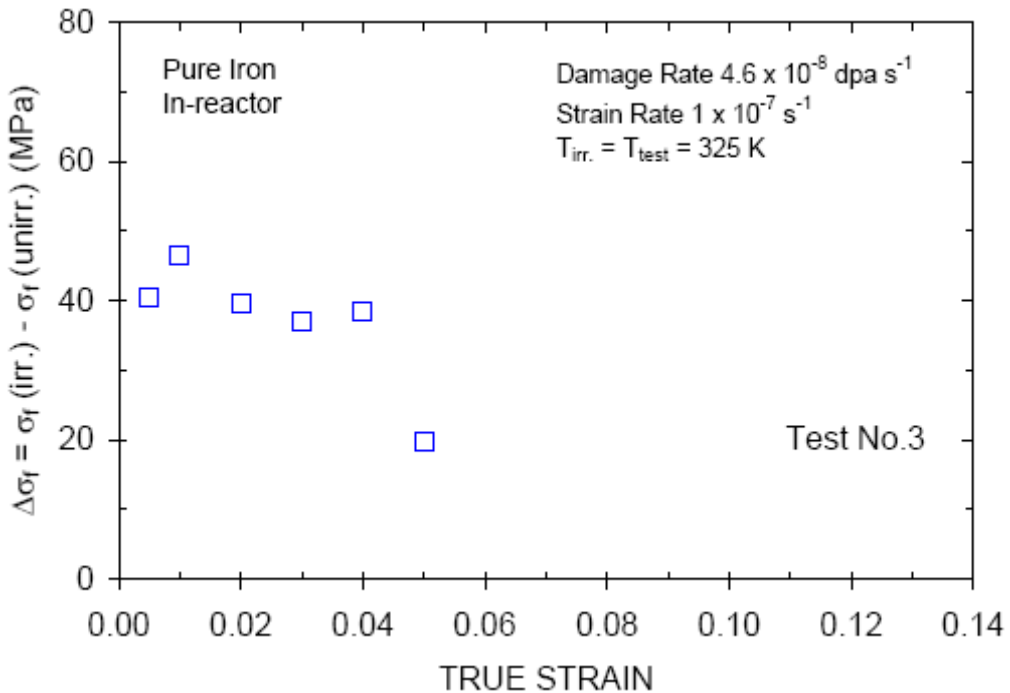
Figure 11. The variation of the increase in post-yield flow stress due to irradiation, \Delta\sigma_f , as a function of true plastic strain for the in-reactor Test No. 3 on pure iron specimen.
