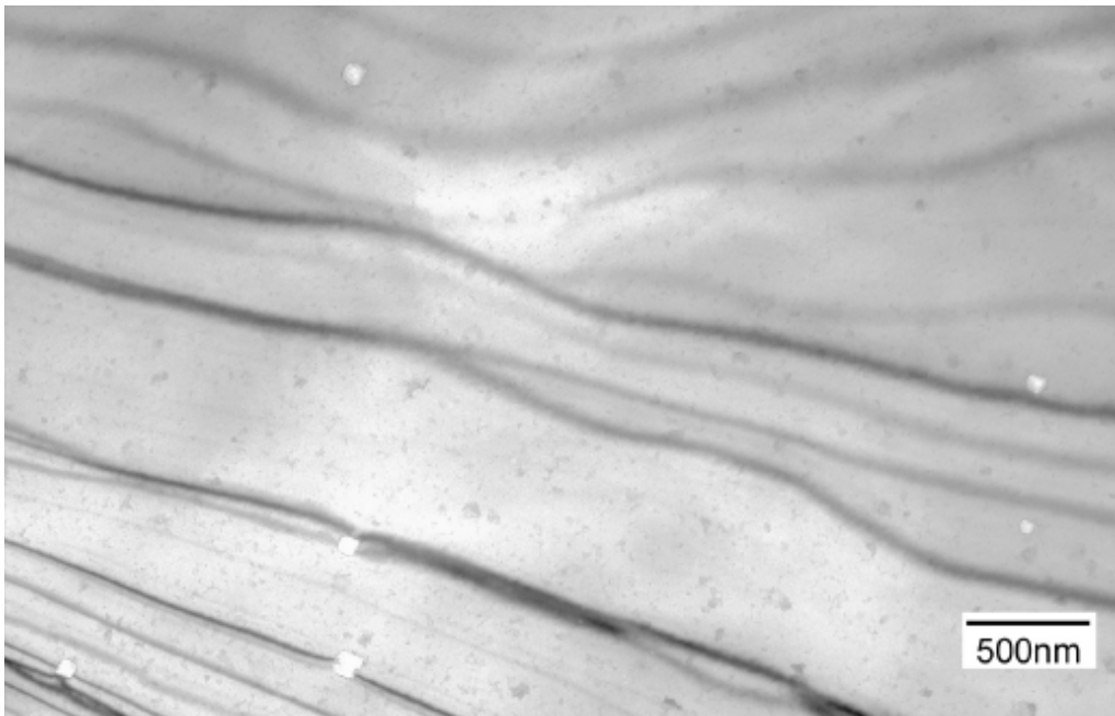
Figure 25. An example of voids formed in the undeformed region of the pure iron specimen used in the in-reactor Test No. 3. These large voids (~89 nm) were found to be present throughout the whole thin foil with a relatively low density ( \sim 1 \times 10^{19} \text{ m}^{-3} ).
