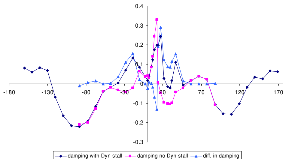
Figure 6-7 Damping shown as a function of AOA. The dark blue line shows the calculations with dynamic stall while the purple line is the calculation without dynamic stall. There is full separation on the entire blade is from about -40 and down and from 50 degrees and up.
