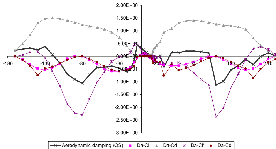
Figure 6-10 The contribution to the damping from the specific terms C_b , C_d , C_l' and C_d' in the 2D quasi-stationary analysis.
