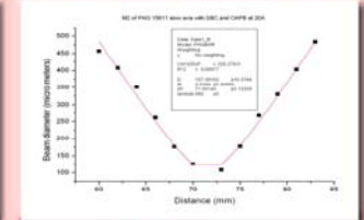
Fig. 7 M^2 along the slow axis
