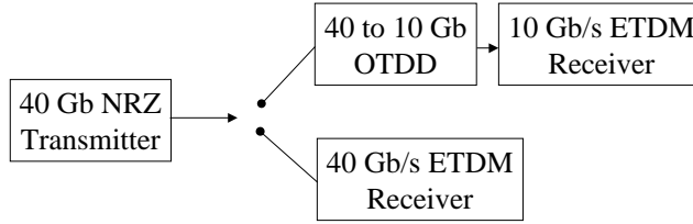
Figure D.1: Overview block diagram of simulation set-up for analysis of OTDD influence on penalty measurements.
