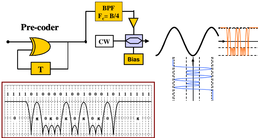
Figure 3.18: Practical implementation of the optical duobinary or PSBT modulation using a chirp free single drive modulator and a X-OR based pre-coder.
