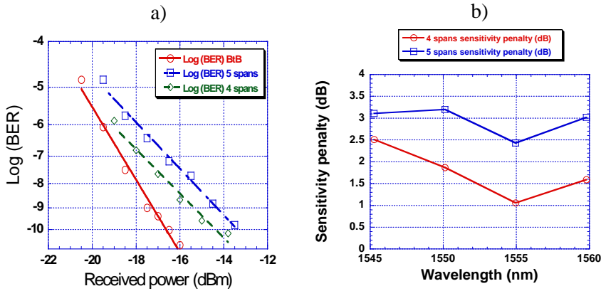
Figure 6.22: BER versus received power measured for the channel situated at 1550.12 nm in the 16 wavelength WDM system transmission experiment over a 400 km standard-SMF link, as presented in Figure 6.16. CSRZ is used as the modulation format. Measurements are shown for the back-to-back WDM situation, after four spans and for the full 400 km link. b) Sensitivity penalty measured for 4 channels.
