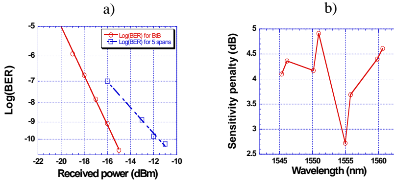
Figure 6.27: a) BER versus received power measured for the channel situated at 1555.75 nm in the 32 wavelength WDM system transmission experiment over a 400 km standard-SMF link using CSRZ as the modulation format. Measurements are shown for the back-to-back WDM situation and for the full 400 km link. b) Sensitivity penalty measured for 8 channels at a BER of 10^{-10} .
