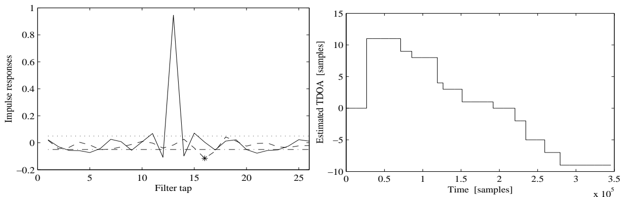
Figure 2. a) Estimated impulse responses h_1 and -h_2 . b) Estimated location for a person walking from side to side.
