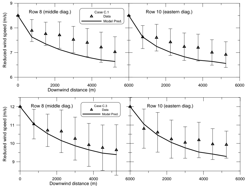
Figure 17. Model predictions at wind direction 222^{\circ} \pm 3^{\circ} compared to data. Free wind speed: 8.5 \text{ m/s} \pm 0.5 \text{ m/s} (top) and 12.0 \text{ m/s} \pm 0.5 \text{ m/s} (bottom).
