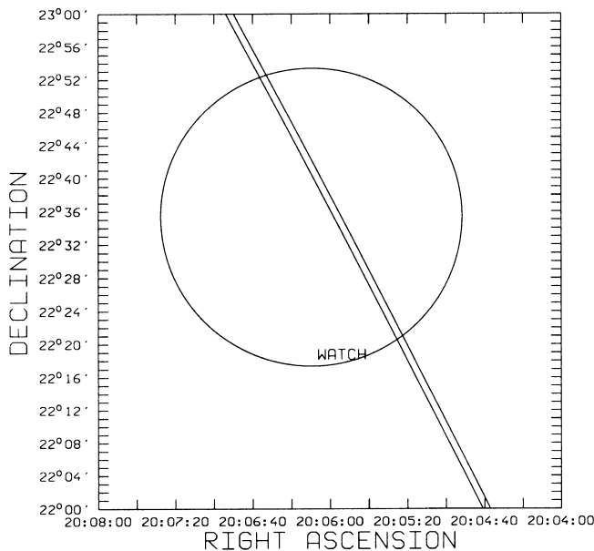
FIG. 14.—IPN annulus ( 3\sigma ) and WATCH error circle ( 3\sigma ) for the burst of 920903 at 23:29.
