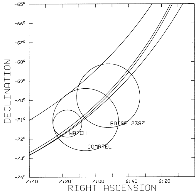
FIG. 20.—IPN 3 \sigma annuli ( Ulysses / BATSE / MO ) and BATSE (1 \sigma ), COMPTEL (1 \sigma ), and WATCH (3 \sigma ) error circles for 930612. The narrow inner IPN annulus and the wider outer IPN annulus intersect outside the figure to form a long error box.
