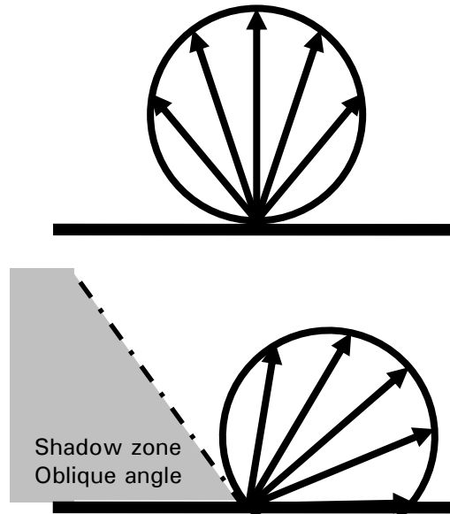
Figur 7. Traditional Lambert directivity at the top and Oblique Lambert at the bottom. Oblique Lambert produces a shadow zone where no sound is reflected. The shadow zone is small if scattering is high or if the incident direction is perpendicular to the wall. On the other hand if scattering is low and the incident direction is oblique then the shadow zone becomes large.
