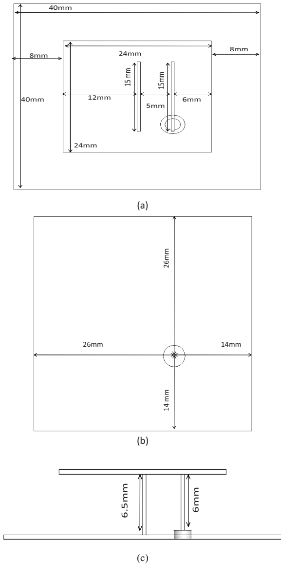
Figure 1: Geometry of the Antenna. (a) Top view, (b) Ground plane (c) Side view.
