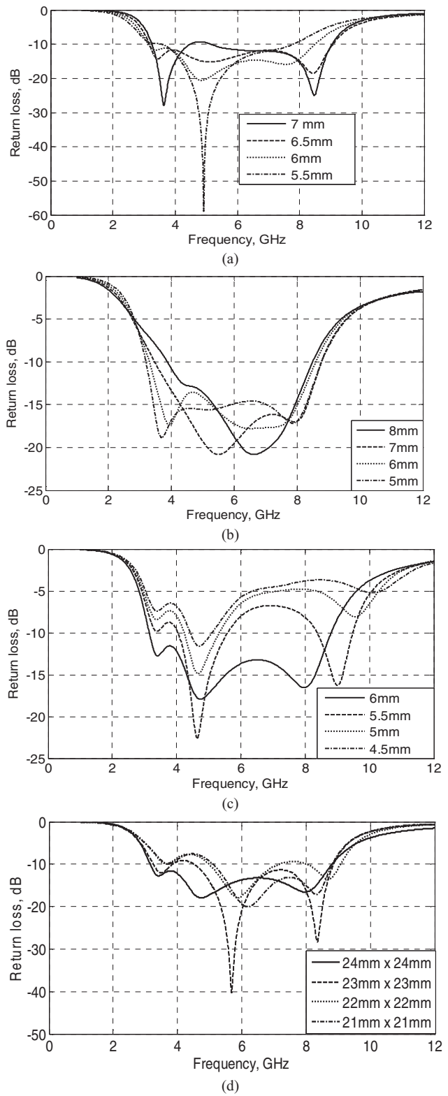
Figure 2: Parametric study. (a) Height of Antenna, (b) Gap between the vertical plates, (c) Height of the feeding plate (d) Size of the radiating patch.
