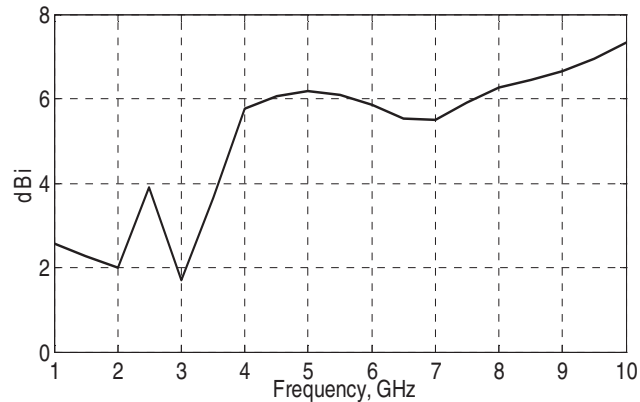
Figure 4: The power gain of the proposed antenna.
