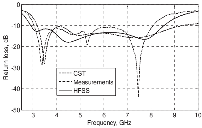
Figure 3: The input return loss of the proposed antenna
