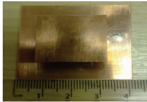
Figure 5: Prototype of the Antenna.
