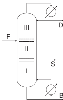
Figure 2.14: Distillation column with side-draw below feed stage.
