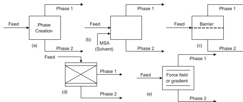
Figure 4.2: Categories of separation mechanisms [Seader and Henley (1998)].
