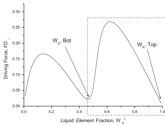
Figure 4.18: Reactive driving force diagram for a binary element system with an indication of the operating range.
