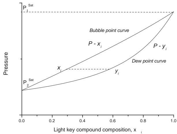
Figure 4.21: A pxy diagram for the compounds i and j at bubble point temperature, T_b .
