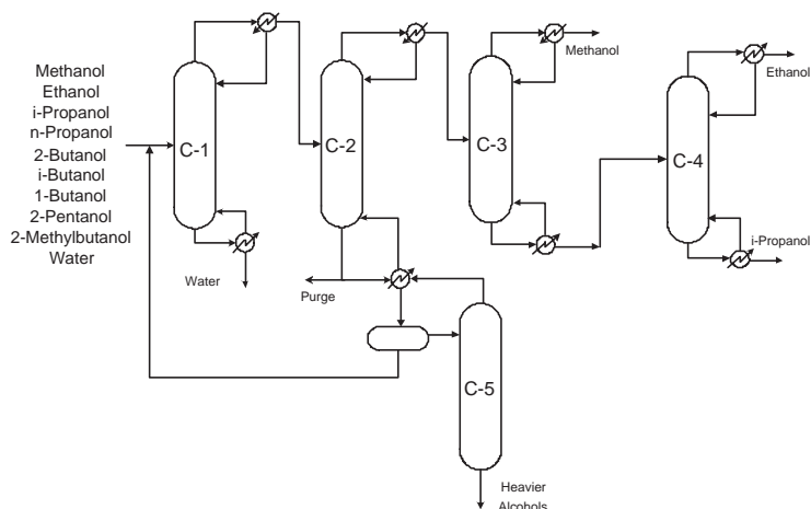
Figure 5.33: Flowsheet for the reverse extractive distillation process proposed by Hunek et al. (1989).
