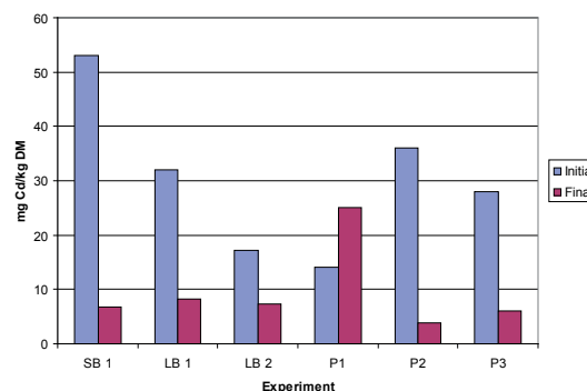
Figure 4: Concentration of Cd in the ash before and after electro-dialytic remediation in different experiments. SB: Small bench scale. LB: Large bench scale. P: Pilot plant. Remediation time: 4 – 10 days.
