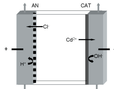
Figure 1: Basic three-compartment cell for electro-dialytic remediation. The ash suspension is placed in the middle compartment (desalination compartment), which is separated from the electrode compartments by ion exchange membranes. AN = anion exchange membrane. CAT = Cation exchange membrane.
