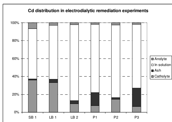
Figure 5: Cd distribution in the different electrolysytic remediation experiments. In percentage of the recovered amount.
