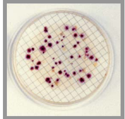
Escherichia coli on modified mTEC agar
