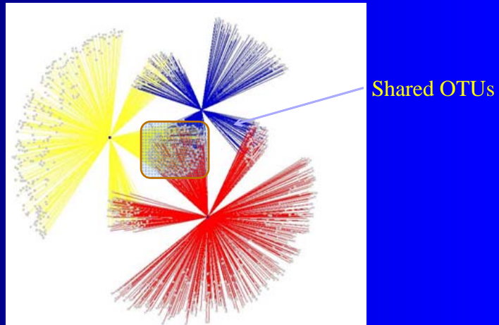
OTU based network analysis of sample A, sample B, AND sample C
