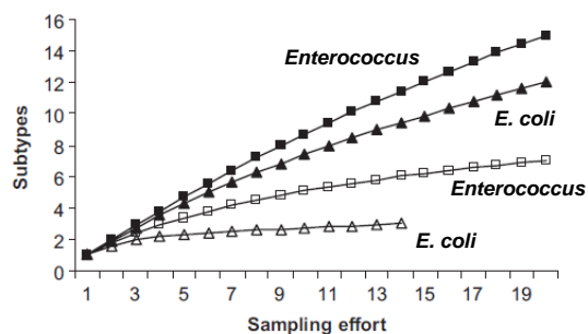
Fig. 2 - Accumulation curves of BOX-PCR fingerprint patterns of indicator bacteria from vault water samples. E. coli sampled after a rain event ( \blacktriangle ) and during dry conditions ( \triangle ); Enterococcus spp. sampled after a rain event ( \blacksquare ) and during dry conditions ( \square ).
