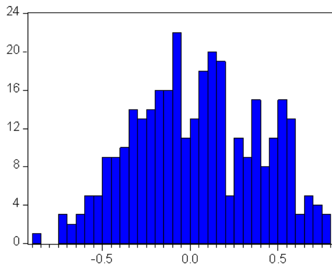
Figure 6: Interprovince correlation of demand shocks 1966-1977
