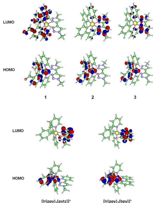
Fig. 5 Plots of HOMO and LUMO orbitals for the ground states of complexes 1 to 3 and [Ir(ppy) 2 (L)] + (L = pytz, bpy).
