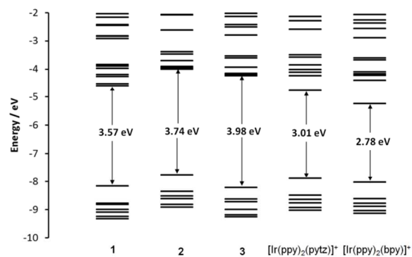
Fig. 6 Energy level diagram for the calculated molecular orbitals of the complexes 1 to 3 and [Ir(ppy) 2 (L)] + (L = pytz, bpy).
