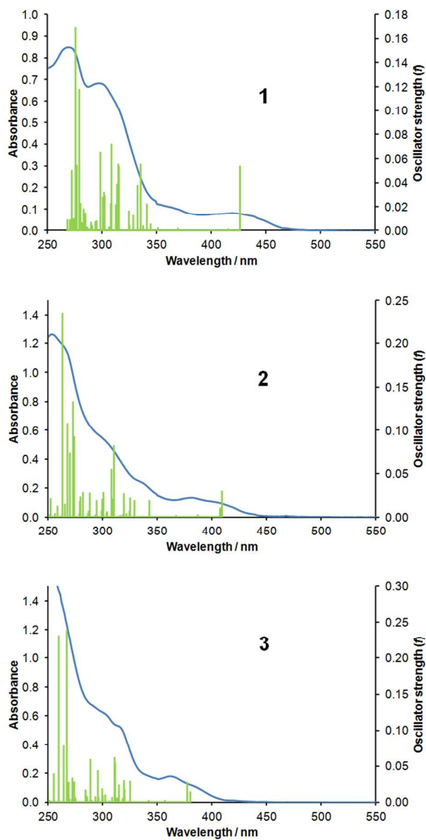
Fig. 7 Overlaid experimental absorbance and calculated TDDFT spectra for complexes 1 to 3. 190x360mm (96 x 96 DPI)
