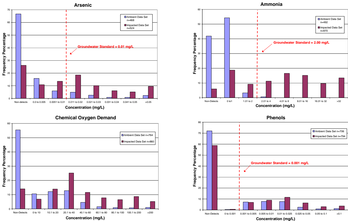
Figures 4a- 4d. Frequency percentage histograms showing differences between ambient and impacted data sets for four parameters which are frequently undetected. Non-detects are grouped together in a single bin to the left of the detected values.
