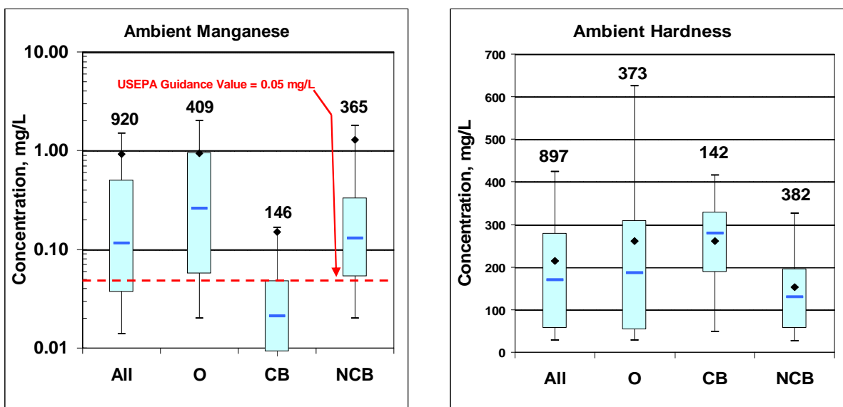
Figures 2a and 2b. Box and whisker diagrams showing variability attributable to aquifer type within the ambient hardness and ambient manganese data sets. (Abbreviations: O = overburden, CB = carbonate bedrock, NCB = non-carbonate bedrock) The light blue box encloses the 25 th to 75 th percentiles of the data set. The median is represented by the blue horizontal bar, while the mean is represented by the black diamond. The upper and lower whiskers indicate the 90 th and 10 th percentiles, respectively. The number above each plot is the number of samples. Applicable groundwater quality standards or guidance values are shown as a dashed red horizontal line.
