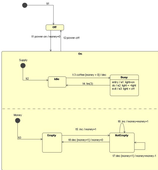
Fig. 1. An example of vending machine state diagram
