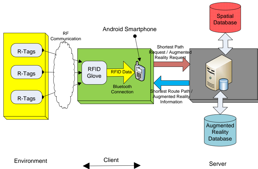
Figure 2.2. FIREGUIDE System Architecture
