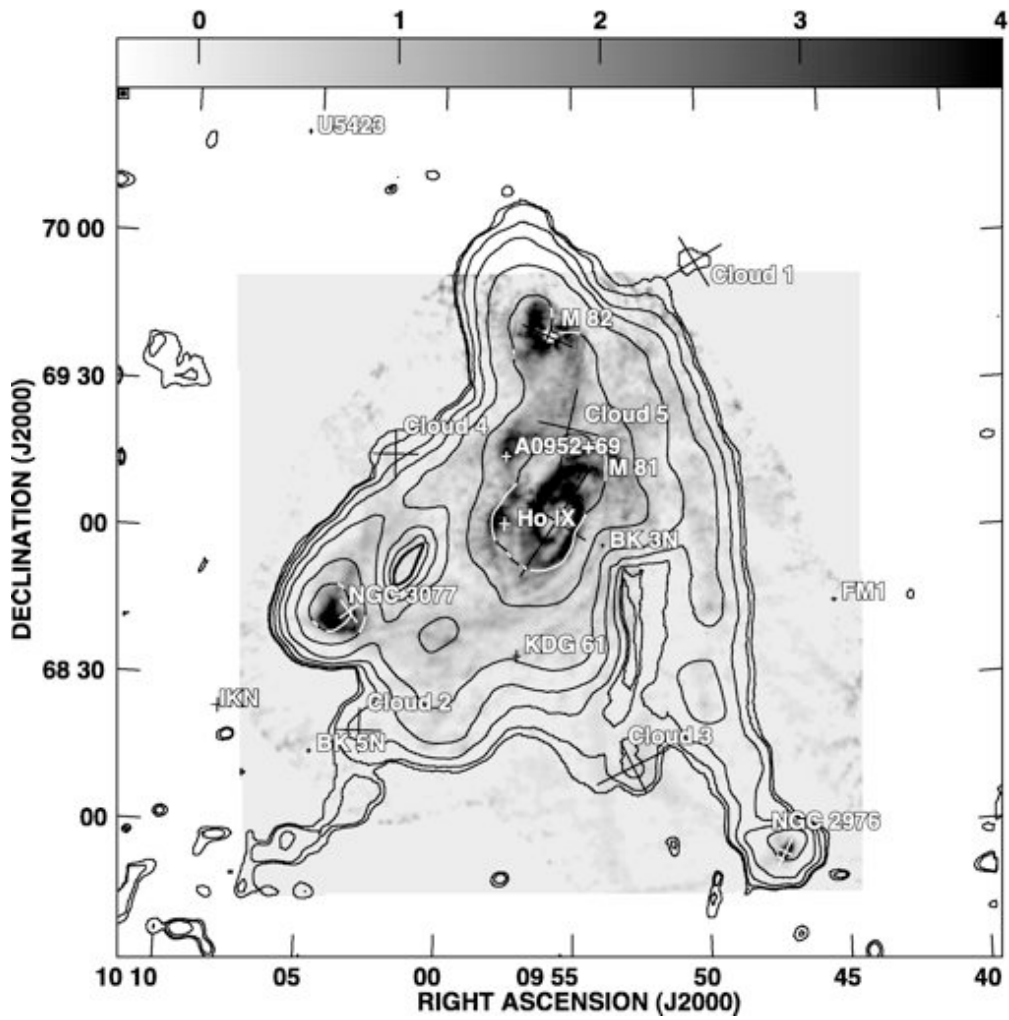
Fig. 1.— The contours show the GBT H I integrated column density map of the field observed. Contours are overlaid at 1500, 3000, 7500, 15000, 30000, 75000, 150000 and 300000 kJy/beam \times km/sec. The velocity range included is -250 to 340 km s^{-1} . The integrated column density map from the VLA observations of Yun et al. (1994) is shown in greyscale over the range -400 to 4000 kJy/beam \times km/sec.
