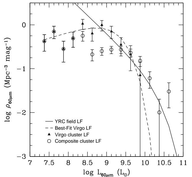
FIG. 7.— The IRAS 60\mu\text{m} LF for the 182 sources in the composite cluster is shown by the open circles. The solid curve denotes the best-fit low luminosity field Schechter LF for the 60\mu\text{m} data of the YRC field sample, normalized to the value of the cluster LF for the bin containing the greatest number of sources. The systematic bias of the cluster LF below that of the best-fit field correlation suggests incompleteness at the low luminosity end. For comparison, we have also shown the IR LF for Virgo cluster sources only, denoted by the filled triangles, along with its best-fit luminosity function indicated by the dashed curve.
