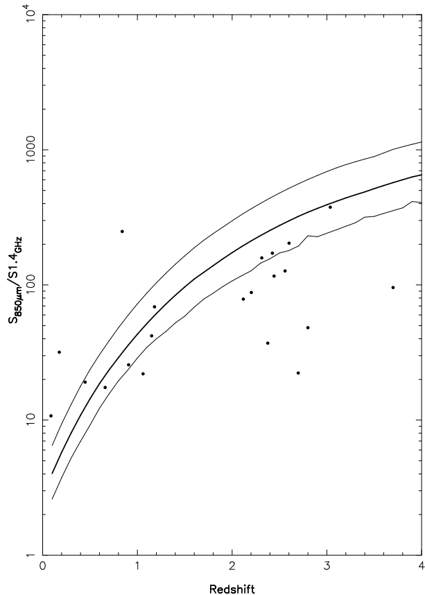
Figure 5. The ratio of 850\mu\text{m} flux to 1.4-GHz flux versus redshift. The lines show predictions of how this flux ratio should depend on redshift for star-forming galaxies using the method described in Dunne, Clements and Eales (2000) and in the text. The thick line shows the median prediction of the templates and the thin lines show \pm 1\sigma predictions based on the range of predicted values at each redshift. The points show SMSs with spectroscopic redshifts and radio detections. The data are from Eales et al. (2000), Smail et al. (2000), Ivison et al. (2002), Chapman et al. (2002, 2003), Simpson et al. (2003) and this paper.
