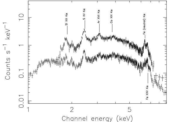
Figure 4. Comparison of accumulated source (lower) and diffuse X-ray emission (upper) spectra for the central enhancement above the surrounding background (see text).
