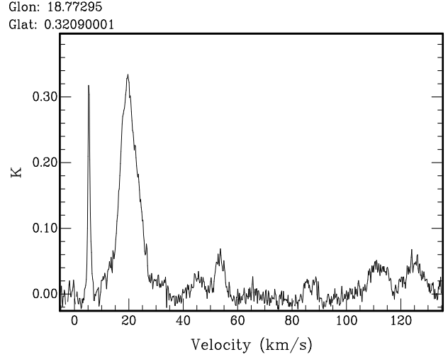
Fig. 4. The average 13 CO spectrum over the full velocity range in the direction of G18.8+0.3.
