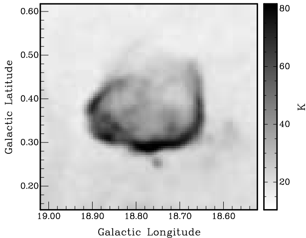
Fig. 1. The figure shows the VGPS continuum image of G18.8+0.3 at 1420 MHz.
