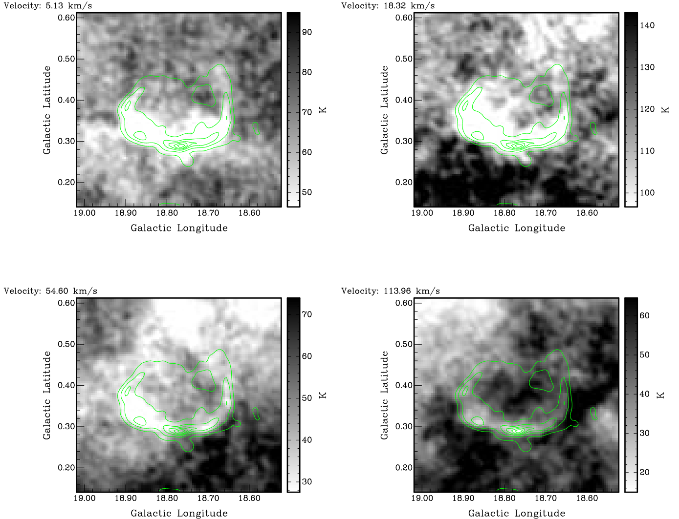
Fig. 2. The maps of HI emission for 4 channels: 5, 18, 54 and 114 \text{km s}^{-1} , respectively. These maps have superimposed contours (28, 48, 68, 80, 90, 100 K) of 1420 MHz continuum emission chosen to show the SNR.
