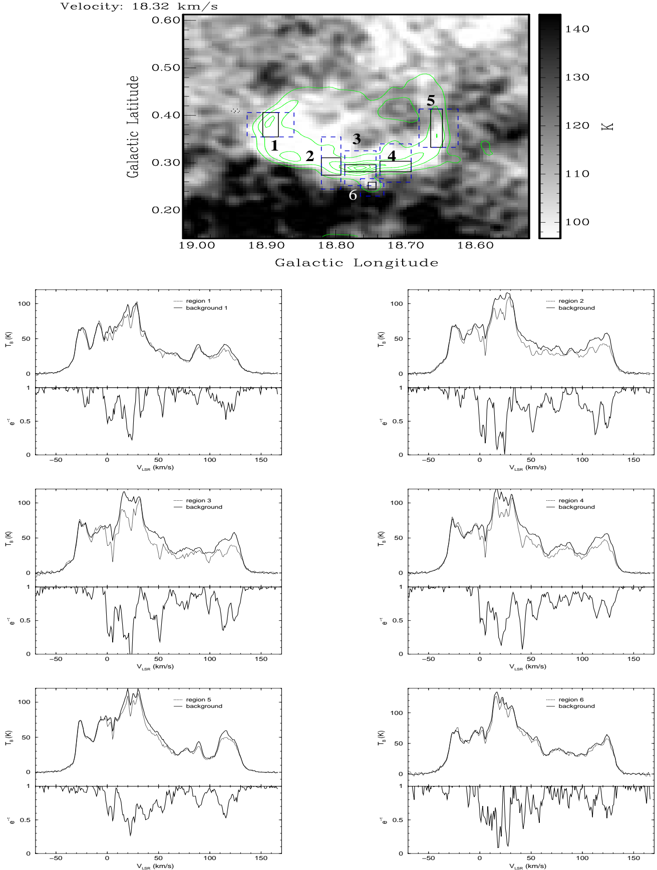
Fig. 3. HI image of G18.8+0.3 from a single channel at 18.3 \text{ km s}^{-1} (top row). The six other panels show the HI spectra, extracted from boxes 1, 2, 3, 4, 5 and 6 shown in the first panel. The HI emission and absorption spectra clearly show absorption features at 1, 5, 11, 24, 27, 51, 98, 113, 126 \text{ km s}^{-1} .
