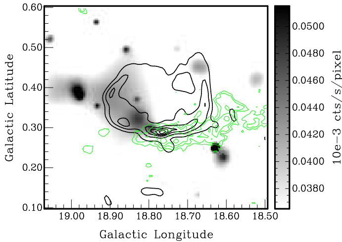
Fig. 6. The ROSAT PSPC intensity image of G18.8+0.3 in the hard band (0.5-2.4 keV). The intensity is adaptively smoothed using csmooth to achieve a signal-to-noise ratio of \sim 3 . The image has superimposed on contours of ^{13}\text{CO} emission (green line: 0.6, 0.9, 1.4, 2.1 K) and 1420 MHz continuum emission as Fig. 2. The units of the intensity are 10^{-3} counts \text{s}^{-1} pixel ^{-1} (1 pixel= 0.25' \times 0.25' )
