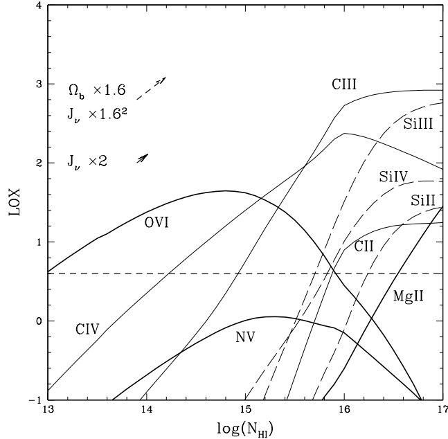
Figure 1: LOX as a function of HI column density for 9 selected absorption lines from carbon (CIV(1548), CIII(977), CII(1335), thin solid lines), silicon (SiIV(1394), SiIII(1206), SiII(1260), dashed lines), and OVI(1032), NV(1243), and MgII(2796) (bold solid lines). The solid arrow indicates the direction and magnitude of changes to the curves if J_\nu is doubled, keeping everything else constant, while the dashed arrow indicates the effect of changing the baryonic density while adjusting J_\nu to keep the mean flux decrement of the spectrum constant (see [11]). The horizontal dashed line indicates LOX=0.6, roughly corresponding to the detection limit in the best available spectra.
