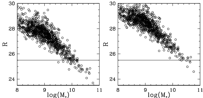
Figure 3: Stellar mass vs. R , without dust (left panel) and with dust (right panel).
