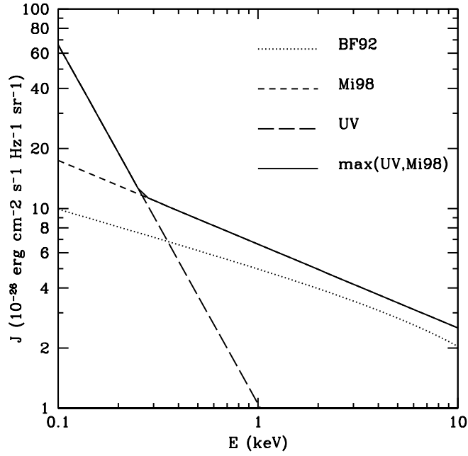
Fig. 1.— The X-ray and UV background spectra used in our calculations. The dotted line shows the BF92 spectrum, eq. (2). The short-dashed line, largely obscured by the solid line, shows the Mi98 spectrum, eq. (1). The long-dashed line shows the UV background spectrum of eq. (3), based on Shull et al. (1999). For most calculations, we take the maximum of the UV and Mi98 spectra, as shown by the solid line. For calculations involving oxygen ions, we also performed calculations with the BF92 spectrum for comparison.
