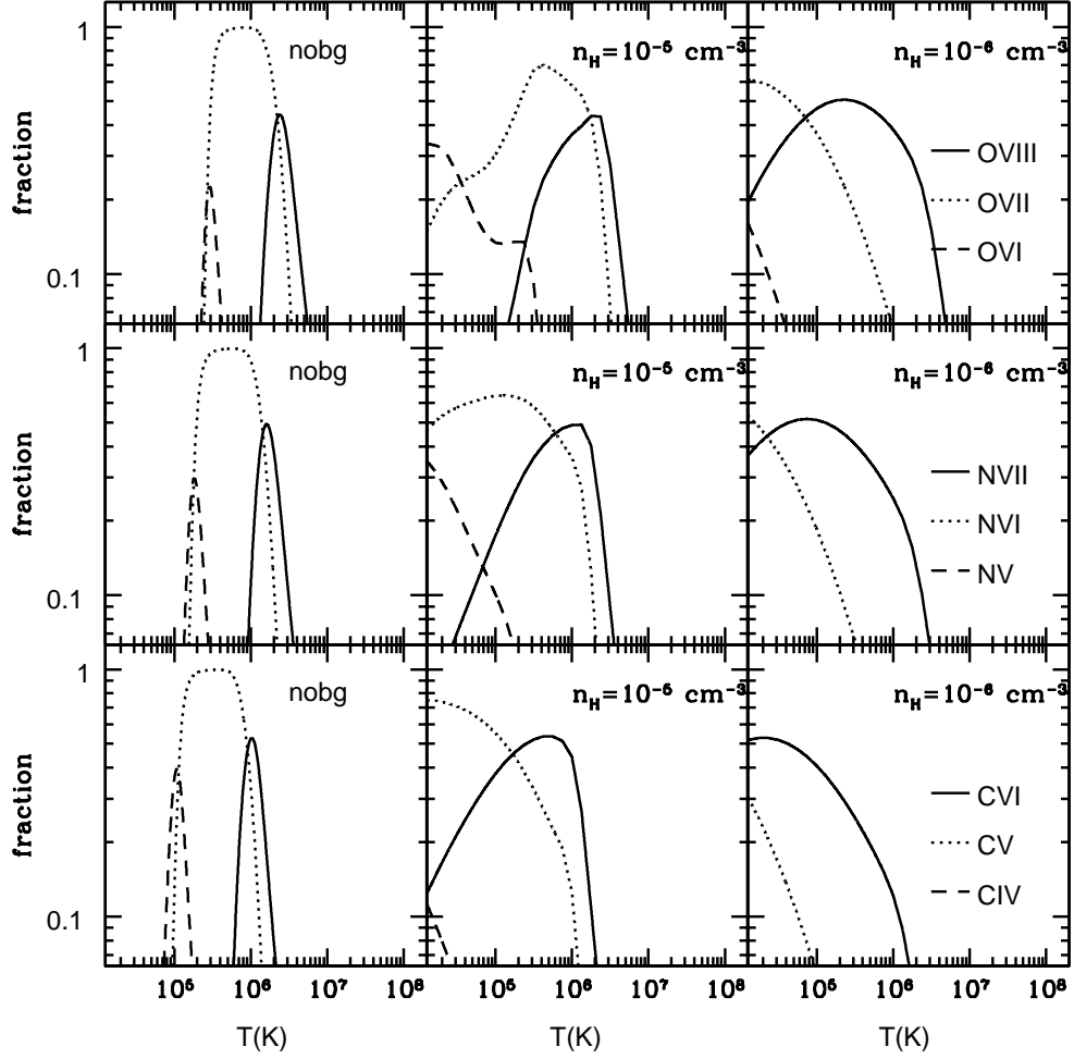
Fig. 2.— Ionization fractions of oxygen (top row), nitrogen(middle row), and carbon (bottom row) as a function of temperature. Left-hand panels show collisional ionization only. Central and right-hand panels show ionization fractions including photoionization by our standard X-ray + UV background (solid line of Fig. 1), for densities n_H = 10^{-5} \text{ cm}^{-3} ( \delta = 60 ) and n_h = 10^{-6} \text{ cm}^{-3} ( \delta = 6 ), respectively.
