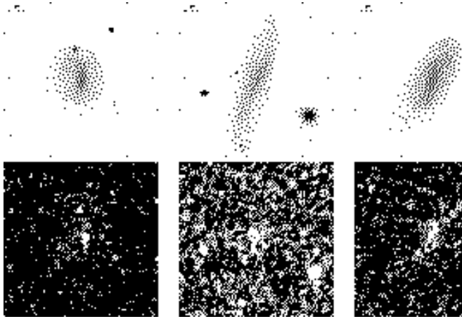
Figure 4. Examples of three bright ( r \leq 14.5 mag) LSBs from MGSphot-only without matches in 2MASS. From left to right, the J2000.0 coordinates are (09:08:51.02,+03:26:54.0), (15:04:30.15,-00:51:04.8) and (12:11:19.92,+01:29:32.2). For each case, we show the colour image from SDSS (top) and the 2MASS K -band image from the same region of sky (bottom). These large, bright galaxies are too low-surface-brightness to be detected by the 2MASS pipeline. Images are 101'' on a side, east is to the left, and a 10'' line is given in the upper left of each optical image from SDSS.
