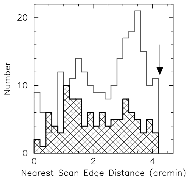
Figure 2. Distribution of distances from the nearest image scan edge for bright MGSphot+spec sources not detected by 2MASS in either the XSC or PSC. Each 2MASS scan is 8.5' \times 6' , thus, the maximum distance to the nearest edge is 4.25' as shown by the arrow. We plot all r \leq 15 (hatched), and a random half of the 15 < r \leq 16 (dark grey outline), nondetections separately. Bright sources missed by 2MASS are uncorrelated with the scan boundaries.
