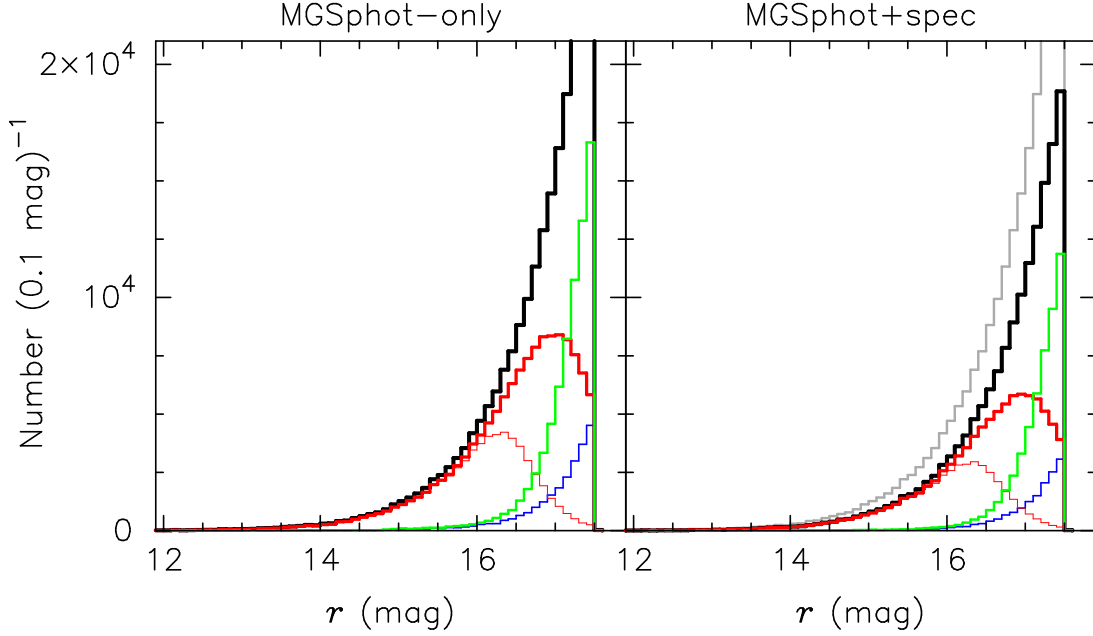
Figure 1. Apparent r -band Petrosian magnitude distributions (black) for the MGSphot-only ( N = 227,614 ) and MGSphot+spec ( N = 156,788 ) primary samples selected from DR2 and limited to r \leq 17.5 mag. In each panel, we show the related subsamples from our cross correlation with the 2MASS XSC (red) and PSC (green); sources without 2MASS counterparts are shown in blue. For comparison, we plot the MGSphot-only distribution in grey in the right panel. Thin red lines denote K \leq 13.57 magnitude-limited XSC samples. All magnitudes are corrected for Galactic extinction following Schlegel et al. (1998).
