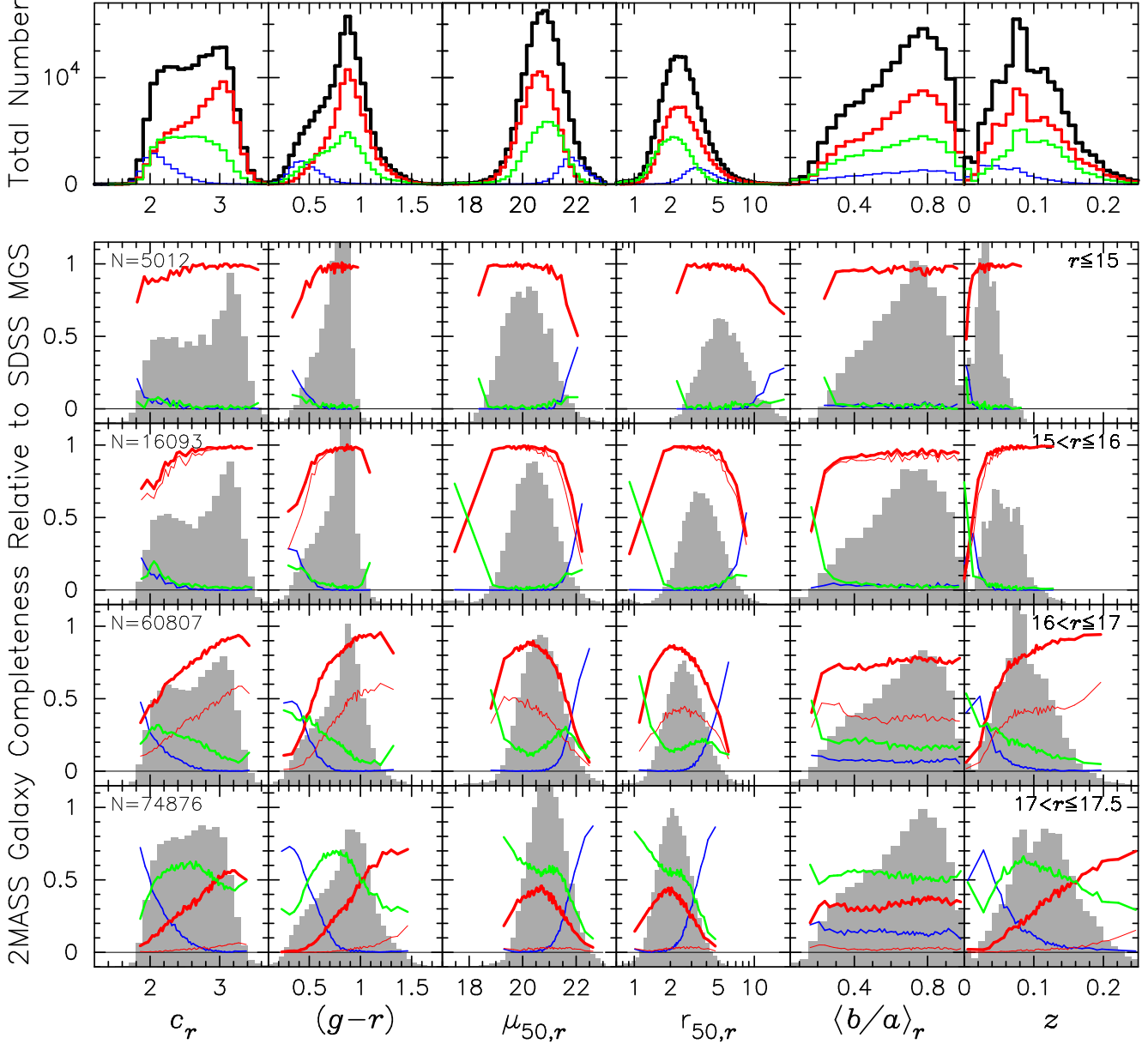
Figure 6. Top row: Observed optical property distributions for the SDSS “main” spectroscopic galaxy selection (MGS phot+spec ; see text for details) limited to have extinction-corrected Petrosian magnitudes brighter than r = 17.5 . Shown from left to right are r -band concentration given by c_r = r_{90,r}/r_{50,r} , (g-r) model colour, half-light r -band surface brightness in \text{mag}/\text{arcsec}^2 , Petrosian half-light radius in arcseconds ( r -band), average r -band axis ratio b/a (see §2.3), and spectroscopic redshift z . In each panel, we plot the total sample (black) of 156,788 galaxies with photometric and spectroscopic properties from DR2, and the subsamples from our cross correlation with the 2MASS XSC (thick red, N = 89,742 ) and PSC (green, N = 51,716 ). In addition, we show the subsample of 15,330 galaxies without 2MASS counterparts (blue). Lower panels: Completeness of 2MASS galaxies with respect to the SDSS spectroscopic sample (MGS phot+spec ) as a function of six fundamental parameters. The completeness functions (CF, see text for details) are given for four different r magnitude cuts corresponding to 95%, 90%, 50%, and 10% minimum XSC completenesses per interval (see Fig. 3). We indicate the total number of galaxies per bin in the left-most panel. The thin red line shows the K \leq 13.57 magnitude-limited XSC sample, which contains a total of 43,663 galaxies. A thin black line marks zero completeness in each panel, and for each magnitude interval we plot the MGS phot+spec property distributions in relative counts (grey histograms).
