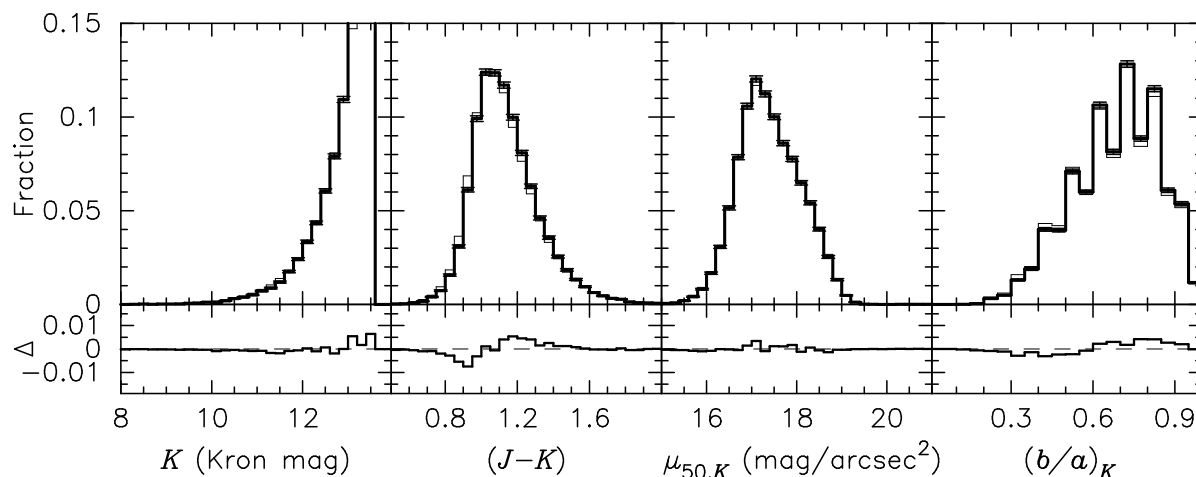
Figure 5. Comparison of two selections of 2MASS galaxies with K \leq 13.57 mag (97.5% completeness): (1) the 548,132 XSC objects outside of the Galactic plane ( |b| > 20^\circ ) with galaxy-like colours of 0.1 \leq (J - K) \leq 2.5 (thin line), and (2) the 43,663 XSC galaxies matched to the r \leq 17.5 DR2 spectroscopic sample (bold line). In each panel we compare the DR2 region and overall high-latitude relative distributions for four primary parameters: (from left to right) K -band Kron magnitude, (J - K) colour, K -band mean surface brightness within r_{50,K} , and K -band axis ratio. For each parameter, the difference (DR2–high-latitude) between the relative fractions is given at the bottom of each panel. We show the Poisson errors per bin for the 2MASS-SDSS matched subsample distributions, which are smaller typically than the per-bin differences. The subsample of K_c \leq 13.57 2MASS galaxies with DR2 counterparts is representative of the full 2MASS XSC outside of the Galactic plane.
