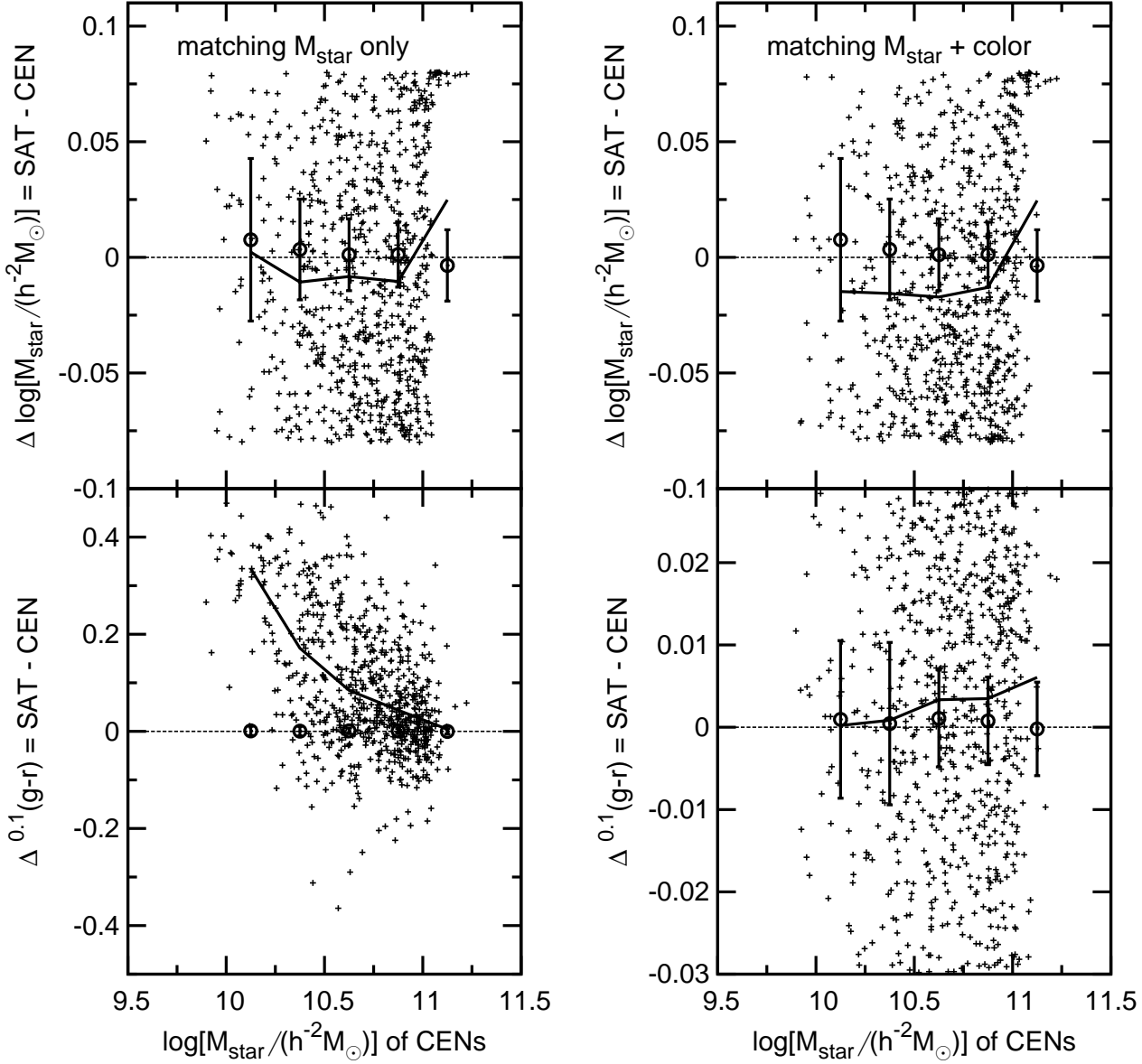
Figure 2. The difference of M_{\text{star}} ( upper panels ) and colour ( lower panels ) between matched CENs and SATs as a function of CEN M_{\text{star}} . The left column shows the differences for the SAT sample S1, which is matched with our CEN sample only in stellar mass, while the right column shows the SAT sample S2, which is matched with our CEN sample in both stellar mass and colour. The solid line in each panel shows the median of the difference for each 0.25 dex wide M_{\text{star}} bin. For comparison, circles with errorbars show the mean and 3\sigma deviation of the biases in each mass bin from matching the CEN sample to 20 mock samples created from itself with random changes according to measurement uncertainties (see text for details).
