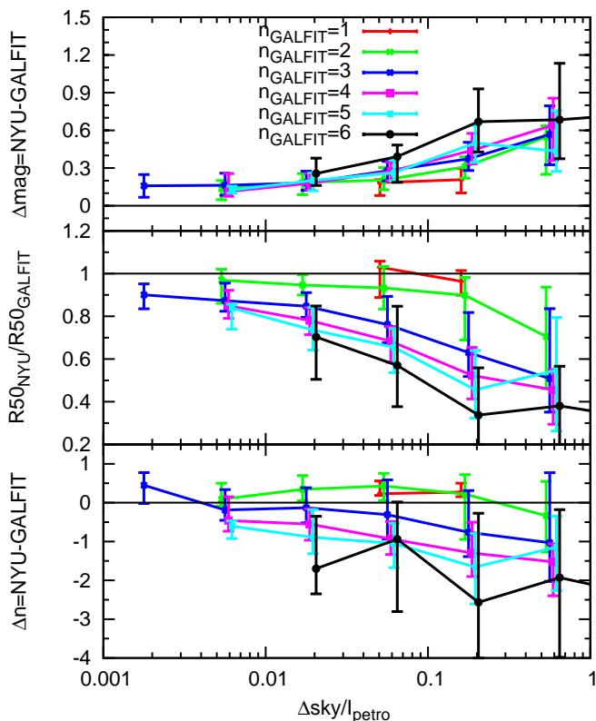
Figure A2. The NYU-VAGC discrepancies shown in Figure A1 as a function of sky difference, divided into GALFIT Sérsic index bins as shown by the colour coding. Here the sky difference is expressed by the ratio between \Delta_{\text{sky}} = \text{local sky} - \text{global sky} and the average Petrosian surface brightness (Petrosian quantities are directly drawn from SDSS tables).
