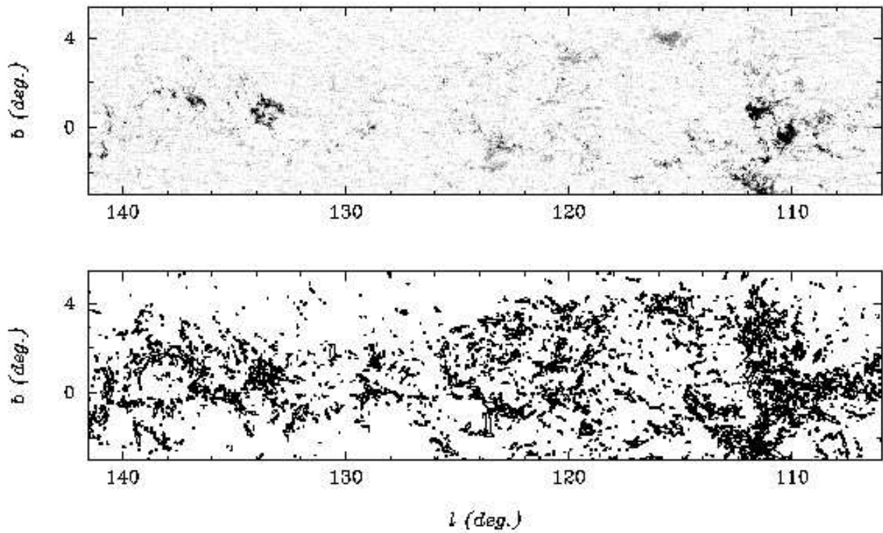
Fig. 1.— (top) An image of ^{12}\text{CO} J=1-0 integrated intensity over the velocity interval -110 to -20 km s ^{-1} from the FCRAO CO Survey of the outer Galaxy (Heyer et al. 1998). The halftone ranges from 0 (white) to 20 (black) K km s ^{-1} . (bottom) The positions, sizes, and orientations of identified objects approximated as ellipses.
