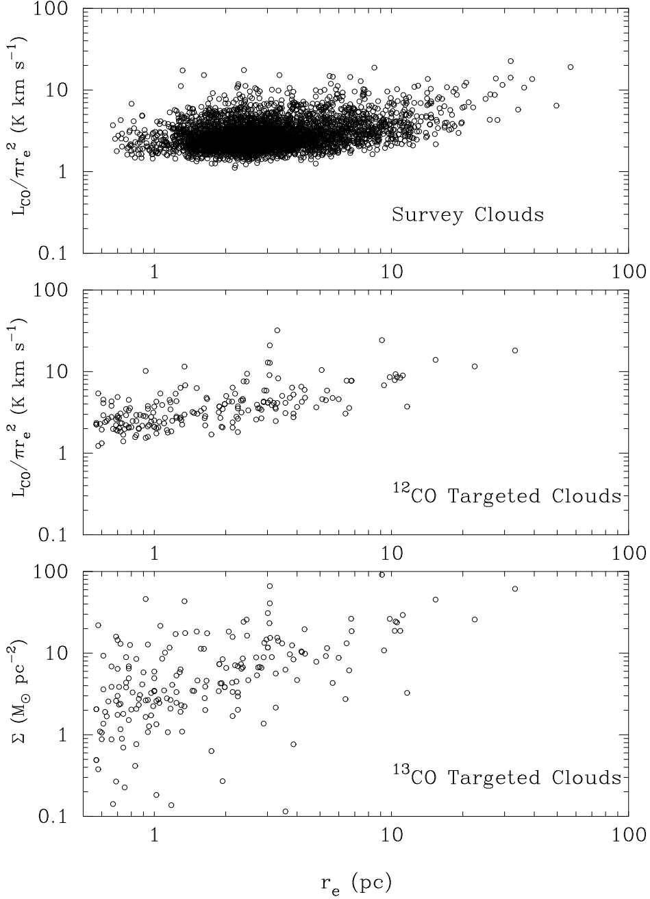
Fig. 10.— (top) The variation of mean CO integrated intensity averaged over the area of the cloud with the effective cloud radius for the sample of Survey clouds. (middle) The variation of mean CO integrated intensity averaged over the area of the cloud with the effective cloud radius for the sample of targeted clouds. (bottom) The mass surface density of objects within the targeted clouds derived from ^{13}\text{CO} observations.
