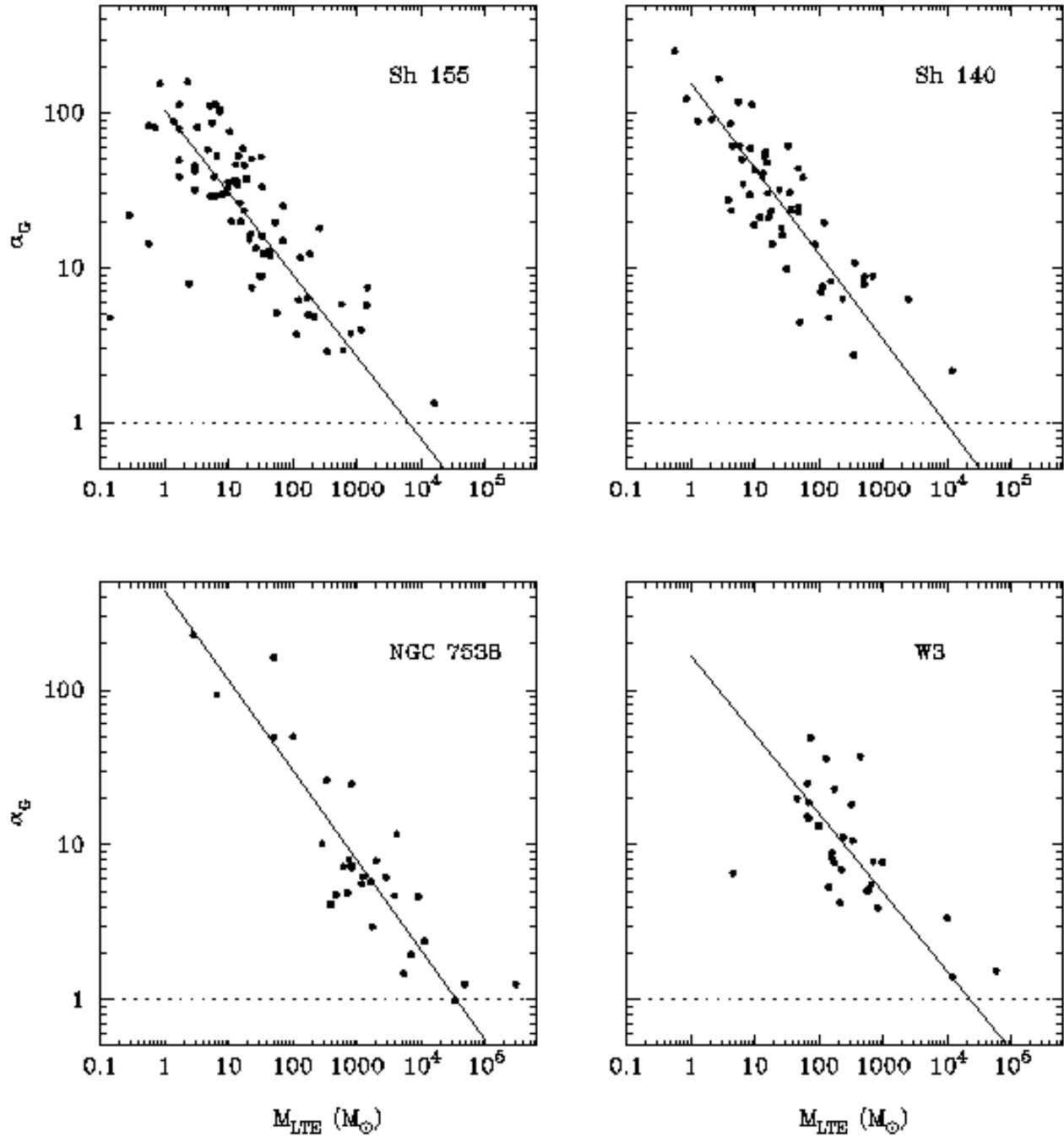
Fig. 8.— The variation of the gravitational parameter, \alpha_G , derived from ^{13}\text{CO} observations for clumps within four targeted giant molecular cloud complexes in the outer Galaxy.
