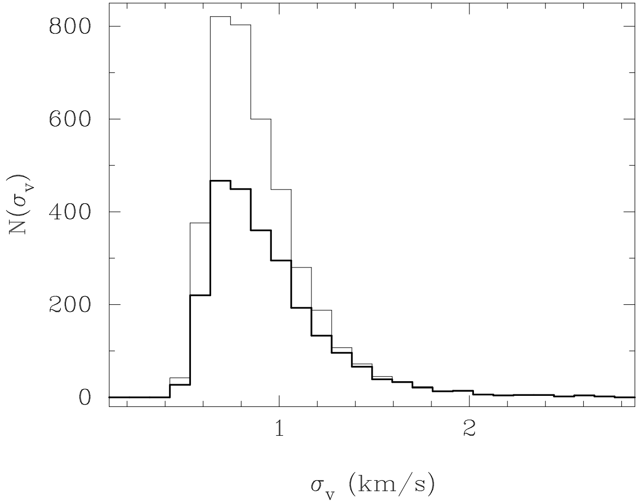
Fig. 5.— The number distribution, N(\sigma_v) of measured velocity dispersion. The heavy solid shows the distribution of velocity dispersion for objects with a peak antenna temperature > 3.5 K for which the velocity dispersions are well determined.
