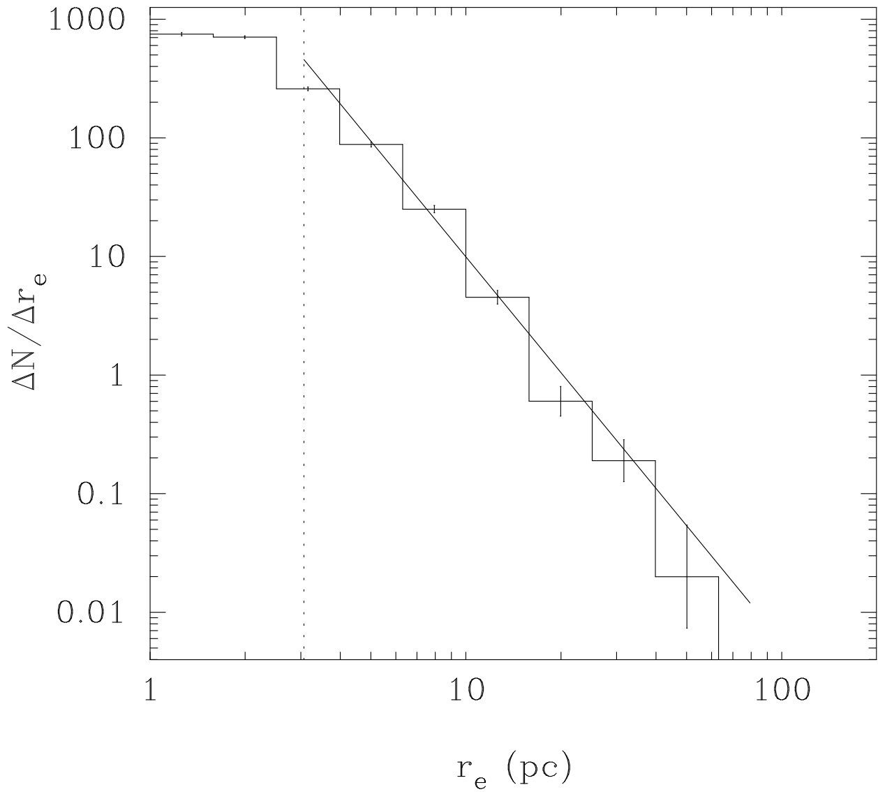
Fig. 4.— The size distribution, \Delta N / \Delta r_e , for the identified objects. The detection limit of r_e at a distance of 10 kpc is 3.1 pc. The power law fit to bins above this limit (solid line) is \Delta N / \Delta r_e \propto r_e^{-3.2 \pm 0.1} .
