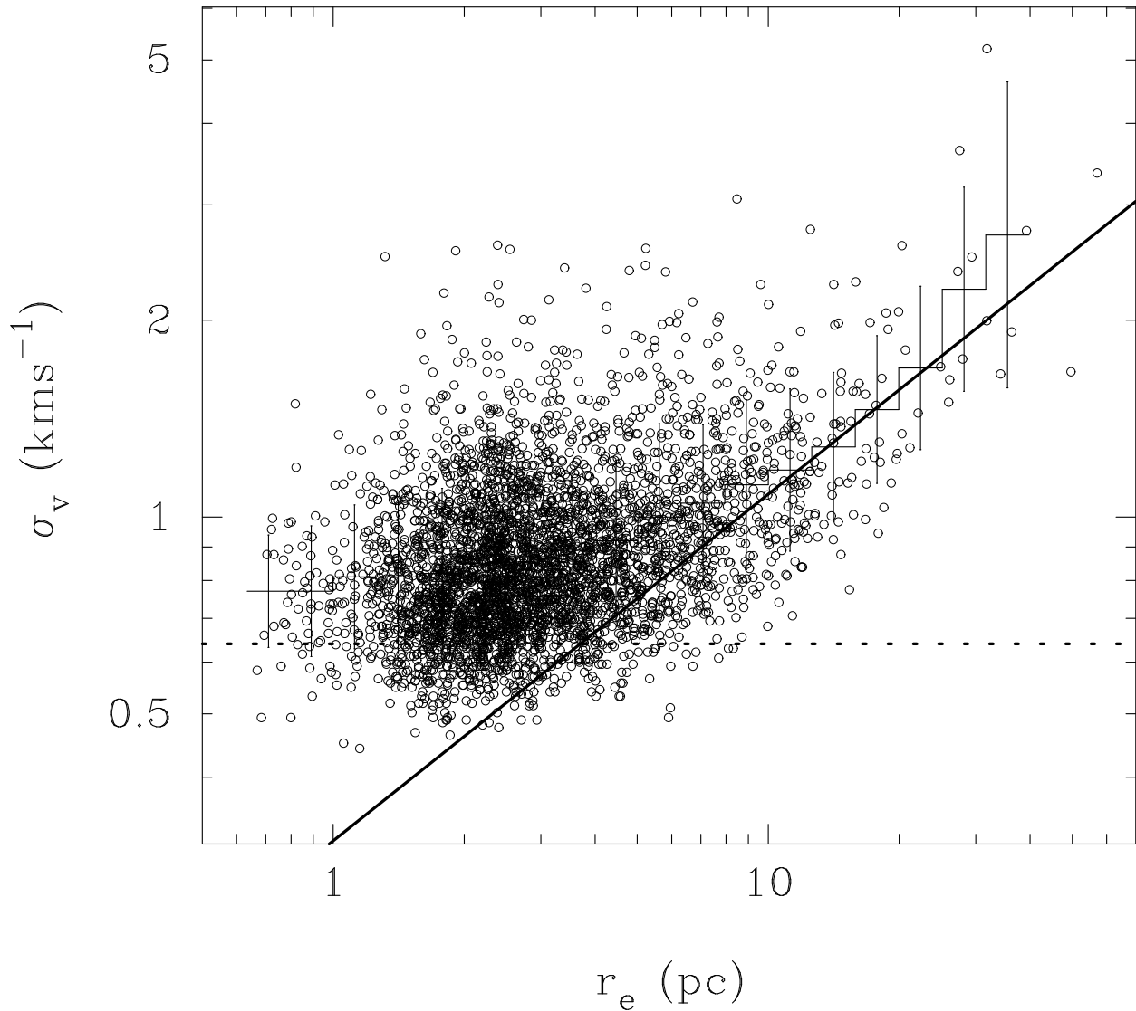
Fig. 6.— The variation of measured velocity dispersion, \sigma_v , and effective size, r_e . The light line shows the mean value within logarithmic bins of r_e and the error bars reflect the dispersion of values about the mean in each bin. The heavy line shows the power law fit to the clouds with r_e > 9 pc. The slope of the power law is similar to that found by Solomon et al. (1987). The horizontal dashed line shows the velocity dispersion to which the measured values are accurate to within 15%.
