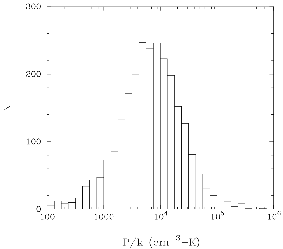
Fig. 12.— The distribution of required external pressures to bind the internal motions of identified molecular regions.
