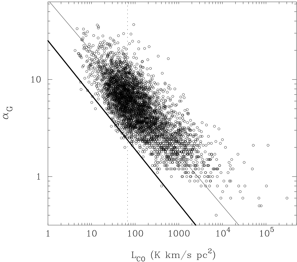
Fig. 7.— The variation of the gravitational parameter, \alpha_G , with CO luminosity. The dotted vertical line denotes the detection limit of L_{CO} at a distance of 10 kpc. The heavy line shows the minimum value of \alpha_G to which the decomposition is sensitive due to the observational selection effect which excludes narrow line clouds.
