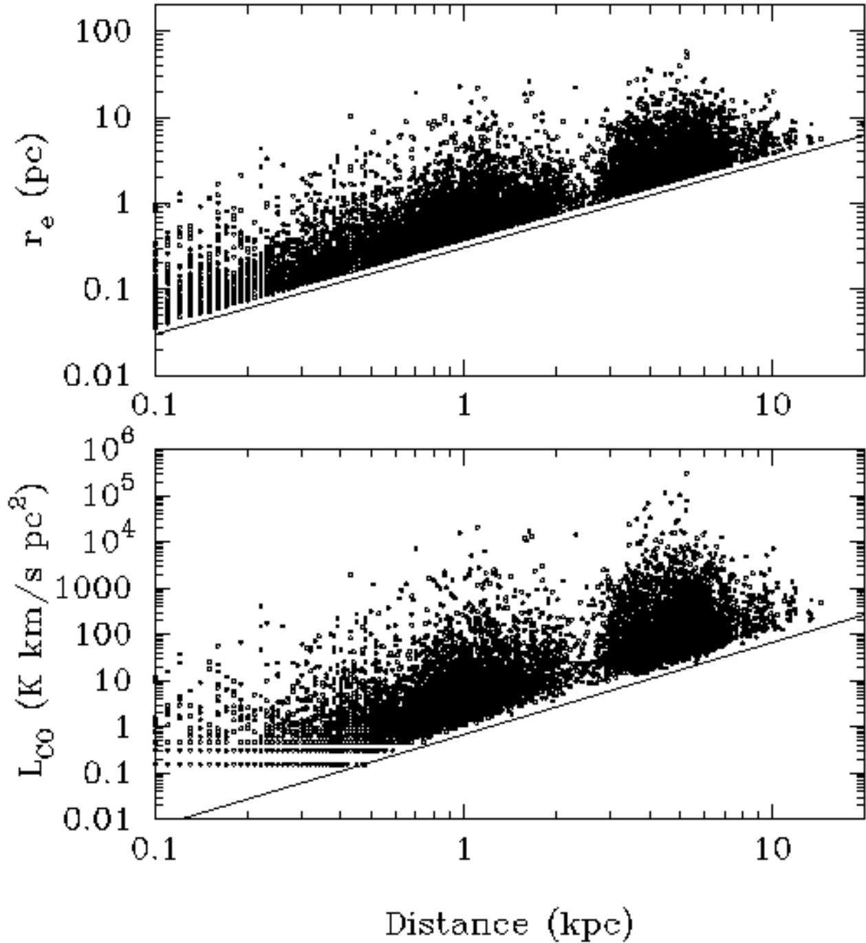
Fig. 2.— (top) The effective radius of identified objects as a function of kinematic distance. The lower envelope of points is due to the requirement that an object must be comprised of at least five spatial pixels. (bottom) L_{CO} as a function of distance. The solid line shows the minimum CO luminosity of objects in which the antenna temperature of all associated positions and spectroscopic channels is 1.4 K.
