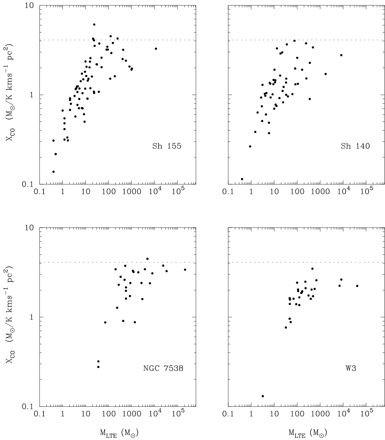
Fig. 9.— The derived CO to H 2 conversion factor for clumps identified within the cloud complexes as a function of mass. For objects with \alpha_G \approx 1 , X_{\text{CO}} is comparable to the value derived from \gamma -ray measurements.
