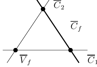
FIGURE 1. Subspaces in \overline{V} for an edge in a 3-dimensional polytope.
