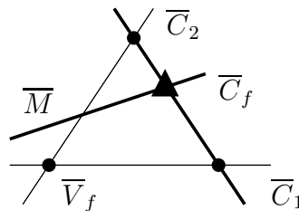
FIGURE 3. Computing T(p, 2) on c_1 .
