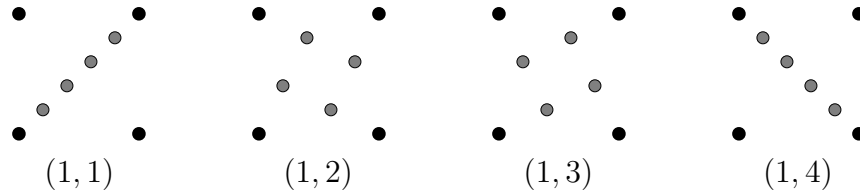
FIGURE 2. Four superlattices giving a nonzero A_s(\alpha, \beta) .
