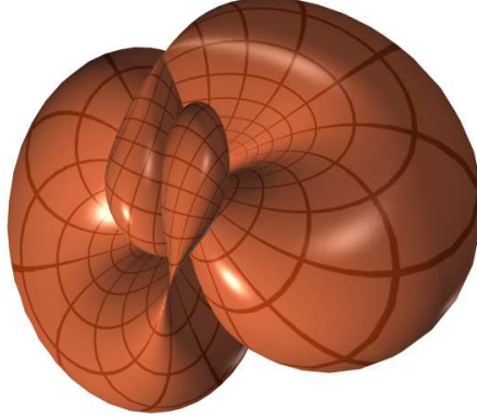
FIGURE 2. Constrained Willmore torus in \mathbb{R}^4 obtained by tangent construction on a twistor projection of an elliptic curve in \mathbb{C}\mathbb{P}^5 , [Hel02]
