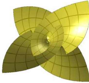
FIGURE 1. Minimal sphere in \mathbb{R}^4 with planar ends obtained by tangent construction on a twistor projection of a holomorphic curve in \mathbb{C}\mathbb{P}^5 , [Hel02]
