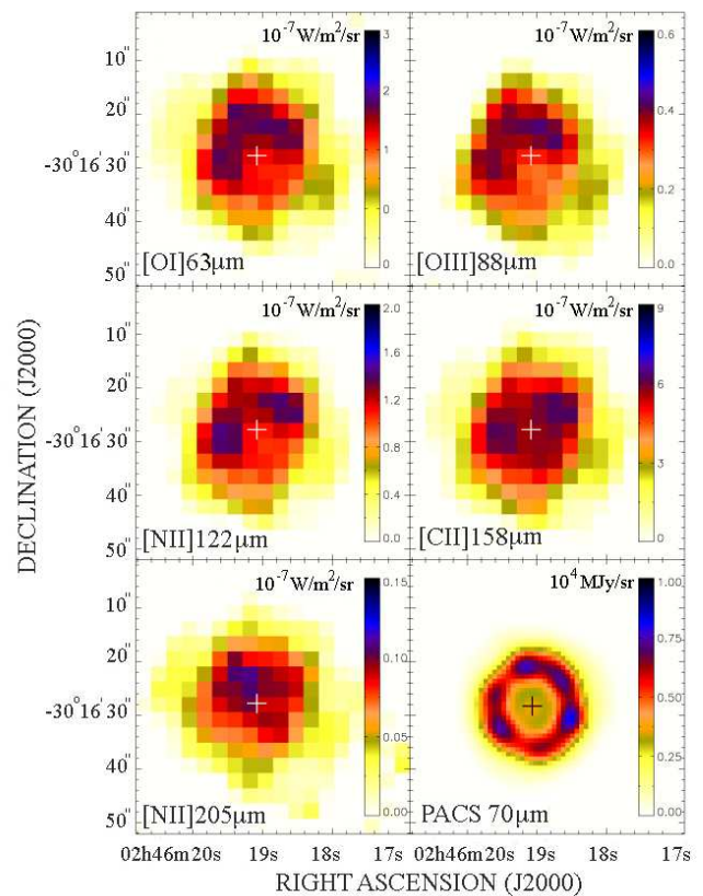
Fig. 2. Spectral maps of the lines observed with PACS at the nuclear position, and an image of the ring at 70 \mu\text{m} with PACS. The maps represent the integrated flux over -500 < v_{\text{sys}} < 500 \text{ km s}^{-1} , with v_{\text{sys}} = 1271 \text{ km s}^{-1} . North is up and East is to the left. In all cases the size of the image is 51'' \times 51'' . The cross marks the location of the radio position of the nucleus.
