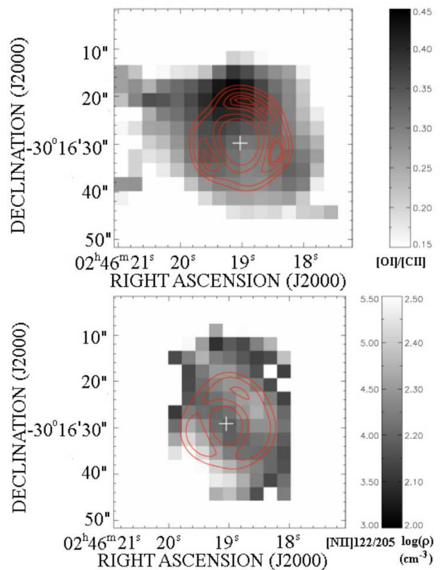
Fig. 5. Top: map of the [OI] 63 \mu\text{m} /[CII] 158 \mu\text{m} ratio. The [OI] 63 \mu\text{m} map was smoothed to match the resolution at 158 \mu\text{m} . Bottom: map of the [NII] 122 \mu\text{m} /[NII] 205 \mu\text{m} ratio. The [NII] 122 \mu\text{m} map was smoothed to match the [NII] 205 \mu\text{m} map. Both maps are overlaid with contours from the PACS 70 \mu\text{m} map, after smoothing to the resolution of each map. All the ratio maps were built from line maps clipped at a 2\sigma level above the noise. The cross marks the location of the nucleus.
