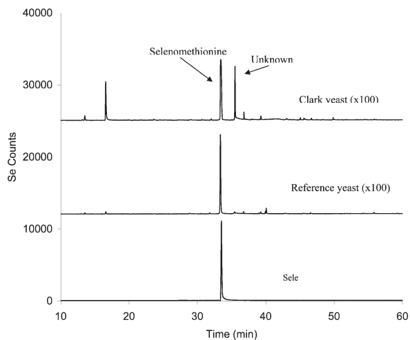
Fig. 4 GC-AED (Se 196 nm) of derivatized selenomethionine, Clark yeast and SelenoExcell ® yeast. Baseline offset for display purposes: Reference yeast trace, baseline is at +12 000 counts; Clark yeast trace, baseline is at +25 000 counts.
