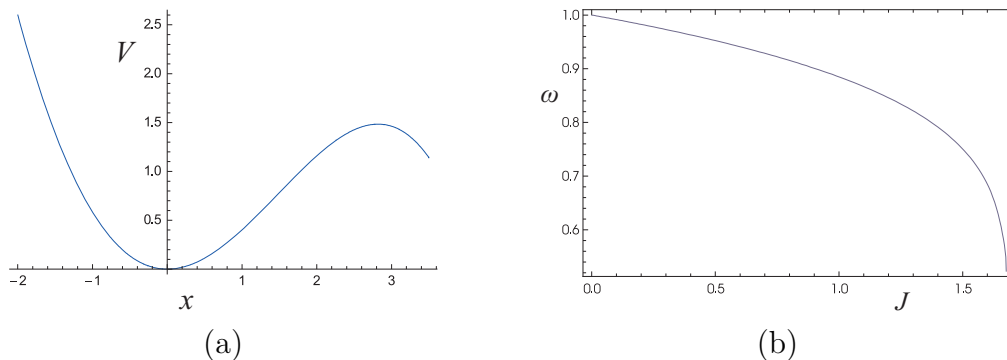
Figure 1. Panel (b) shows the dependence of \omega with respect to J for the specific V(x) of panel (a).
