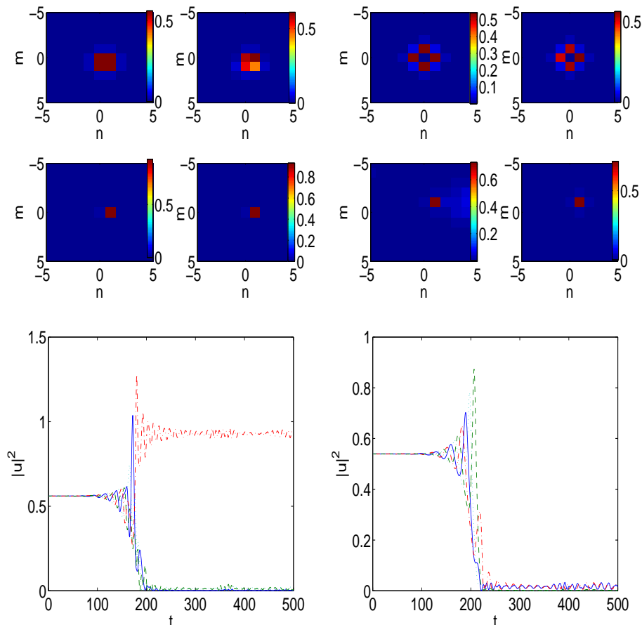
FIG. 10: (Color Online) Same as in Fig. 2 but for the dynamical evolution of the IS (left panels) and the OS (right panels) vortex of topological charge S = 1 . Both cases are shown for C = 0.1 . Both the left and right panels of evolution are for t = 50 , t = 150 (top row), t = 250 and t = 350 (second row) and alongside the bottom panels showing the principal four sites of the vortex they show how the vortices transform themselves into fundamental solitary waves centered on a single site (in the latter case, interestingly, the site of the largest excitation of the ensuing wave is not one among the four principal excitation sites of the original OS vortex).
