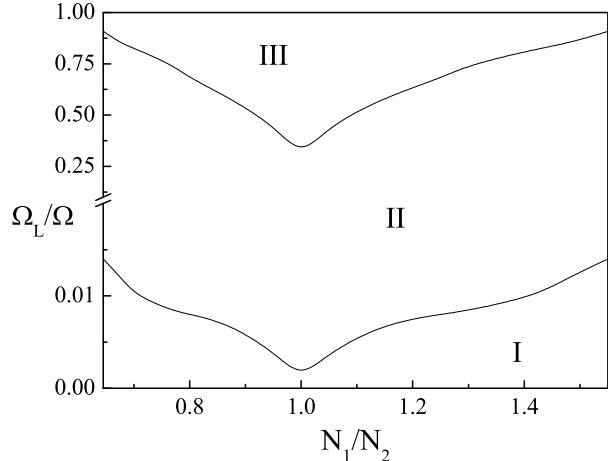
FIG. 8. The region of the stable rotation of the domain-wall crosses, shown in the parameter plane (N_1/N_2, \Omega_L/\Omega) . In region I, the DW cross is quiescent, in region III it is destroyed, while in region II it is rotating in a stable manner. Note that for values of N_1/N_2 outside the interval (0.65, 1.55) the DW crosses are unstable.
