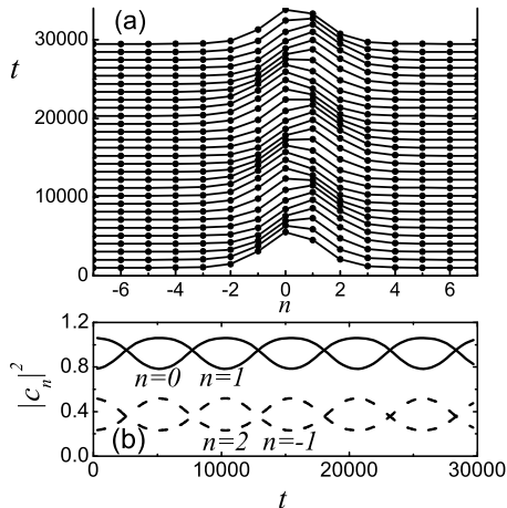
FIG. 6: Pulse in Case 2 ( W_2 = 0 ). (a) Space-time evolution of |c_n(t)|^2 showing the dynamics of the pulse placed at t = 0 asymmetrically with respect to the lattice. The pulse undergoes periodic oscillations in the vicinity of the stable inter-site configuration. (b) Time variation of the norm of the four central particles. Parameters: W_1 = -0.012 , W_2 = 0 , \omega = -0.99 , which corresponds to the point A in Fig. 3.
