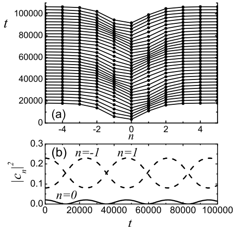
FIG. 8: Kink in Case 2 ( W_2 = 0 ). (a) Space-time evolution of |c_n(t)|^2 showing the dynamics of the kink placed at t = 0 asymmetrically with respect to the lattice. The kink undergoes periodic oscillations in the vicinity of the stable on-site configuration. (b) Time variation of the norm of the central particle and its two nearest neighbors. Parameters: W_1 = 0.012 , W_2 = 0 , \omega = -0.9 , which corresponds to the point B in Fig. 3.
