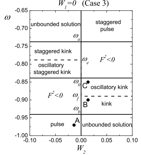
FIG. 5: Parameter plane ( W_2, \omega ) in Case 3 ( W_1 = 0 ) with indicated regions of existence of three types of solitons shown in Fig. 4 and their staggered analogues. The pulse exists for W_2 < 0 and \omega < \omega_b , while the staggered pulse for W_2 > 0 and \omega > \omega_a . The kink exists for W_2 > 0 and \omega_b < \omega < \omega_f , while the staggered kink for W_2 < 0 and \omega_e < \omega < \omega_a . Finally, the oscillatory kink exists for W_2 > 0 and \omega_f < \omega < \omega_0 , while the oscillatory staggered kink for W_2 < 0 and \omega_0 < \omega < \omega_e . Values of special frequencies are given by Eq. (46) and Eq. (48).
