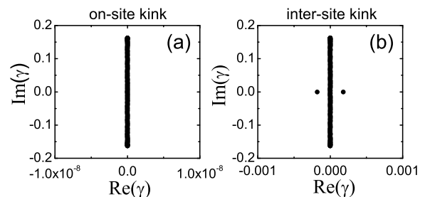
FIG. 11: Spectra of (a) stable on-site and (b) unstable inter-site kinks. The parameters (Case 2): W_1 = 0.012 , W_2 = 0 , \omega = -0.9 correspond to the point B in Fig. 3.
