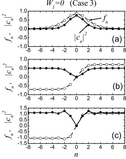
FIG. 4: Equilibrium soliton solutions obtained in Case 3 with W_1 = 0 : (a) pulse, (b) kink, and (c) kink with oscillatory tail, called oscillatory kink. On-site structures are presented here, but inter-site ones can also be constructed. All these solutions can be stable, as it will be shown in Sec. V C. Model parameters corresponding to panels (a) to (c) are depicted by dots in Fig. 5 marked by the capital Latin letters A to C, respectively. Parameters are: (a) W_2 = -0.0136 , \omega = -0.9704 , (b) W_2 = 0.0136 , \omega = -0.9 , (c) W_2 = 0.0136 , \omega = -0.85 .
