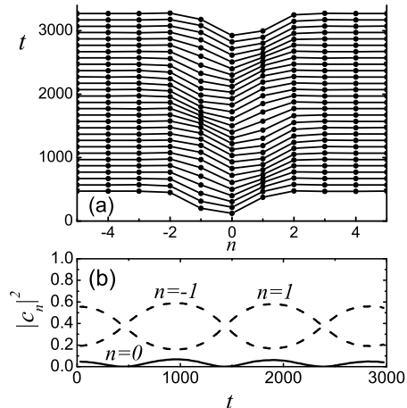
FIG. 9: Kink with oscillatory tail in Case 3 ( W_1 = 0 ). (a) Space-time evolution of |c_n(t)|^2 showing the dynamics of the kink with oscillatory tail placed at t = 0 asymmetrically with respect to the lattice. The kink with oscillatory tail undergoes periodic oscillations in the vicinity of the stable on-site configuration. (b) Time variation of the norm of the central particle and its two nearest neighbors. Parameters: W_1 = 0 , W_2 = 0.0136 , \omega = -0.88 . The kink with oscillatory tail has frequency close to \omega_f = -0.8896 and it becomes unstable far from this line (see Fig. 15).
