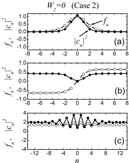
FIG. 2: Equilibrium soliton solutions found in the Case 2 ( W_2 = 0 ): (a) pulse, (b) kink, and (c) anti-dark structure with oscillatory wave structure around the background, hereafter termed wave. On-site structures are presented here, but inter-site ones can also be constructed. Solutions in (a) and (b) can be stable but we were unable to find a stable structure of the form presented in (c) (see Sec. V C). Model parameters corresponding to panels (a) to (c) are depicted in Fig. 3 marked by the capital letters A to C, respectively. Parameters are: (a) W_1 = -0.0112 , \omega = -0.99 , (b) W_1 = 0.0112 , \omega = -0.9 , (c) W_1 = 0.0112 , \omega = -0.75 .
