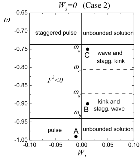
FIG. 3: Parameter plane ( W_1, \omega ) in the Case 2 ( W_2 = 0 ) with indicated regions of existence of three types of solitons shown in Fig. 2 and their staggered analogues. The pulse solution exists for W_1 < 0 and \omega < \omega_b , while the staggered pulse for W_1 < 0 and \omega > \omega_a . The kink and staggered wave can exist for W_1 > 0 and \omega_b < \omega < \omega_c , while the staggered kink and the wave for W_1 > 0 and \omega_d < \omega < \omega_a . The values of special frequencies \omega_a to \omega_d are given by Eq. (46) and Eq. (47).
