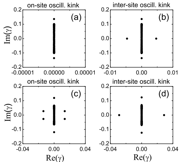
FIG. 15: The top panels show spectra of (a) stable on-site and (b) unstable inter-site oscillatory kinks with \omega = -0.88 . The bottom panels show the same for \omega = -0.85 when both on-site and inter-site oscillatory kinks become unstable. Note that the type of instability in (c) is different from that in (d). In (c) there are two pairs of complex-conjugate eigenvalues, while in (d) there is a pair of purely real eigenvalues. The rest of the parameters are (Case 3) W_1 = 0 , W_2 = 0.0136 .
