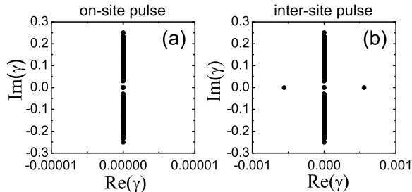
FIG. 13: Spectra of (a) stable on-site and (b) unstable inter-site pulses. Oscillatory motion of the pulse in the vicinity of the on-site configuration is shown in Fig. 6. The parameters (Case 3) W_1 = 0 , W_2 = -0.0136 , \omega = -0.9704 correspond to the point A in Fig. 5.
