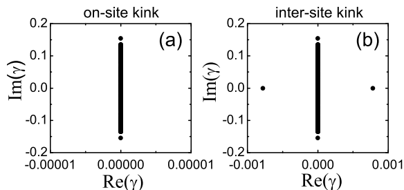
FIG. 14: Spectra of (a) stable on-site and (b) unstable inter-site kinks. The parameter values (Case 3) W_1 = 0 , W_2 = 0.0136 , \omega = -0.9 correspond to the point B in Fig. 5.
