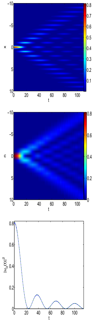
FIG. 1: The top and middle panel show the space-time contour plot of the solution in the PDE of Eq. (1) [top panel] and the discrete model analytical prediction (33) [middle panel]. In the latter case, space is normalized over the period of the linear potential, so that it can be compared with the lattice results. To accentuate the excellent agreement between analytical and numerical results, the bottom panel shows the time evolution of the amplitude at the central site of the configuration compared between the PDE numerical result (solid line) and the discrete equation analytical result of (33) (dashed line). The two are practically indistinguishable .
