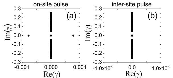
FIG. 10: Spectra of (a) unstable on-site and (b) stable inter-site pulses. The parameters (Case 2): W_1 = -0.012 , W_2 = 0 , \omega = -0.99 correspond to the point A in Fig. 3.
