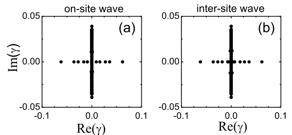
FIG. 12: Spectra of (a) unstable on-site and (b) unstable inter-site wave. The parameters (Case 2): W_1 = 0.012 , W_2 = 0 , \omega = -0.75 correspond to the point C in Fig. 3.
