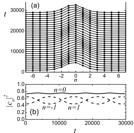
FIG. 7: Pulse in Case 3 ( W_1 = 0 ). (a) Space-time evolution of |c_n(t)|^2 showing the dynamics of the pulse placed at t = 0 asymmetrically with respect to the lattice. The pulse undergoes periodic oscillations in the vicinity of the stable on-site configuration. (b) Time variation of the norm of the central particle and its two nearest neighbors. Parameters: W_1 = 0 , W_2 = -0.0136 , \omega = -0.9704 , which corresponds to the point A in Fig. 5.
