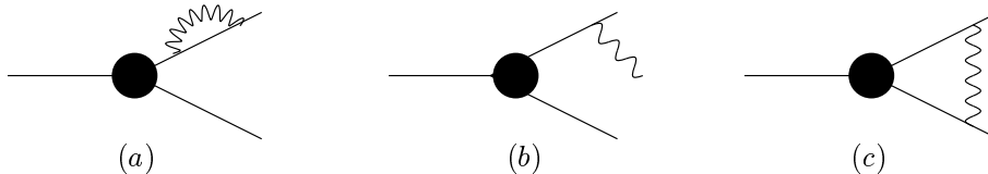
FIG. 1. Electromagnetic contributions relevant for the infrared behavior.
