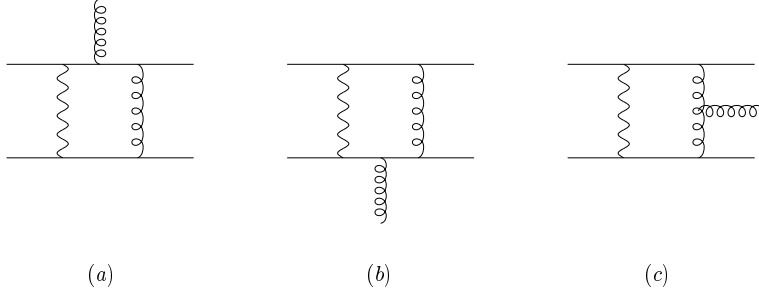
FIG. 3. Gluon radiation from the box diagram.
