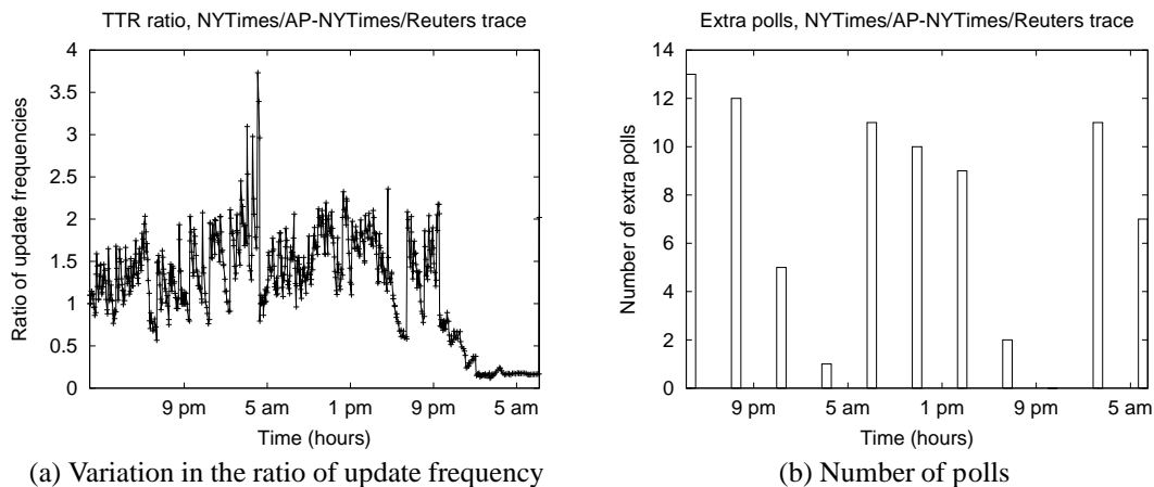
Figure 6. Adaptive behavior of our heuristic for mutual consistency.
