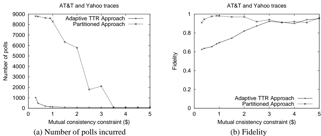
Figure 7. Efficacy of our mutual consistency techniques in the value domain.
