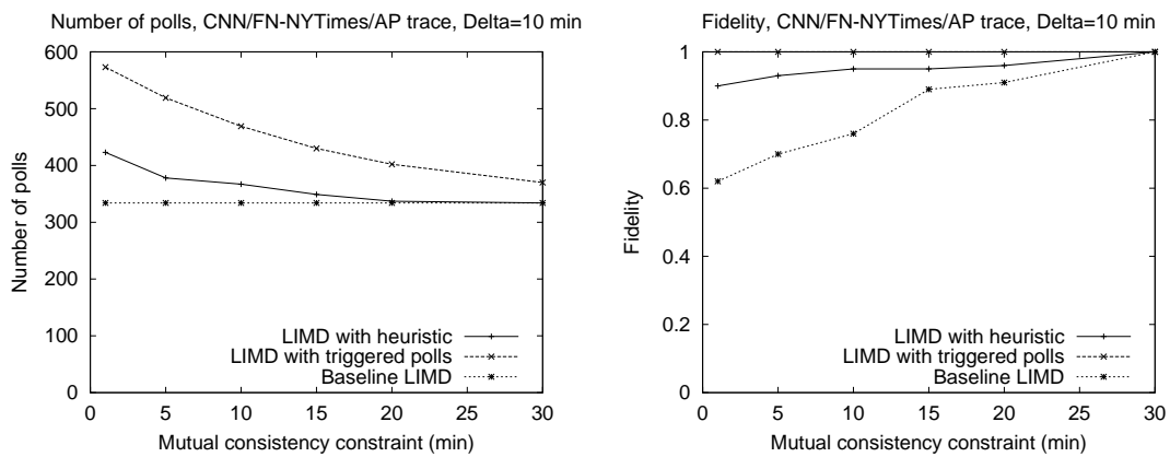
Figure 5. Performance of different mutual consistency approaches
