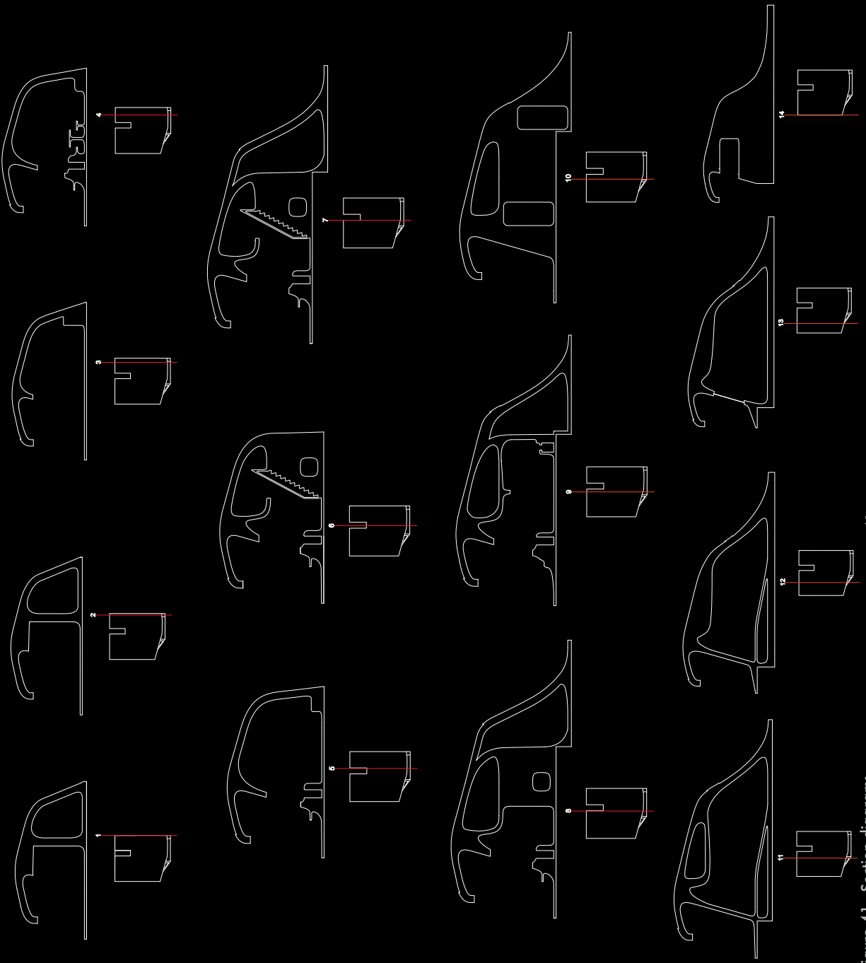
Figure 41 - Section diagrams
