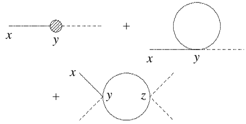
FIG. 1: The leading contributions to the running of the running of the mass m and the coupling \lambda in a \varphi^4 theory. The solid lines represent propagating \psi fields while the dashed lines correspond to the zero mode \phi .
