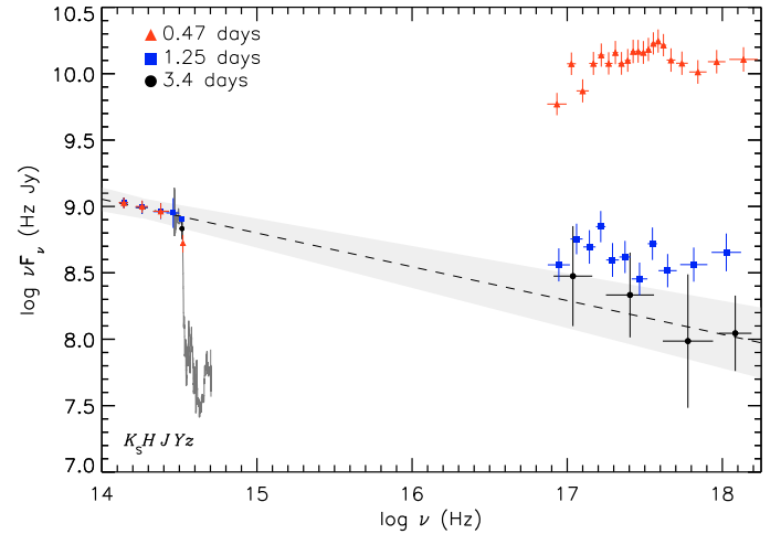
Fig. 2. Near-infrared to X-ray spectral energy distribution of the afterglow of GRB 050904 at 0.47 (red triangles), 1.25 (blue squares) and 3.4 days (black circles) after the burst. The SED at 0.47 and 1.25 days is scaled to the H -band at 3.4 days. The solid grey curve represents the median-filtered optical spectrum at t_0 + 3.4 days. The black dashed line corresponds to a power-law fit to the near-infrared to the X-ray data at 3.4 days with a spectral index \beta = 1.25 \pm 0.05 . The grey shaded area represents the 1\sigma uncertainty on the power-law.
