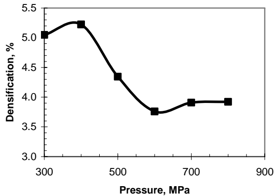
Fig.7. Densification during sintering at 1280°C of Astalloy CrM + 1 % Mn + 0.88 % C samples as a function of compacting pressure. Powder particles were coated with CHS from solution.
