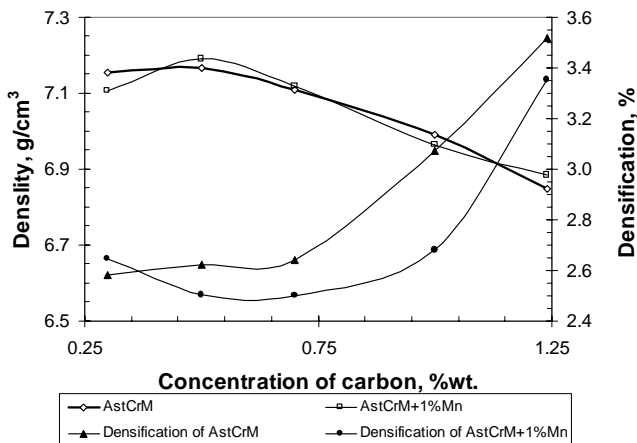
Fig.8. Sintered density (isothermal sintering temperature - 1200°C) and densification of Astalloy CrM and Astalloy CrM + 1 % Mn specimens compacted at 800 MPa as a function of carbon content. Powder particles were coated with CHS from solution.
