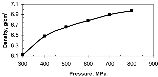
Fig.9. Sintered density (isothermal sintering temperature - 1280°C) of Astalloy CrM + 1 % Mn + 0.88 % C specimens as a function of compacting pressure. Powder particles were coated with CHS from solution.
