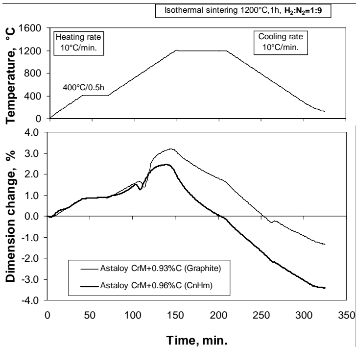
Fig.10. Dilatometric traces for AstCrM + 0.96 % C (coating from solution) and AstCrM + 0.93 % C (graphite) after sintering at 1200°C for 60 min in nitrogen-hydrogen atmosphere 9:1.
