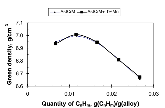
Fig.5. Green densities of Astaloy CrM and Astaloy CrM + 1 % Mn samples as a function of the quantity of C_nH_m addition. Compacting pressure 800 MPa. Powder particles were coated with CHS from solution.
