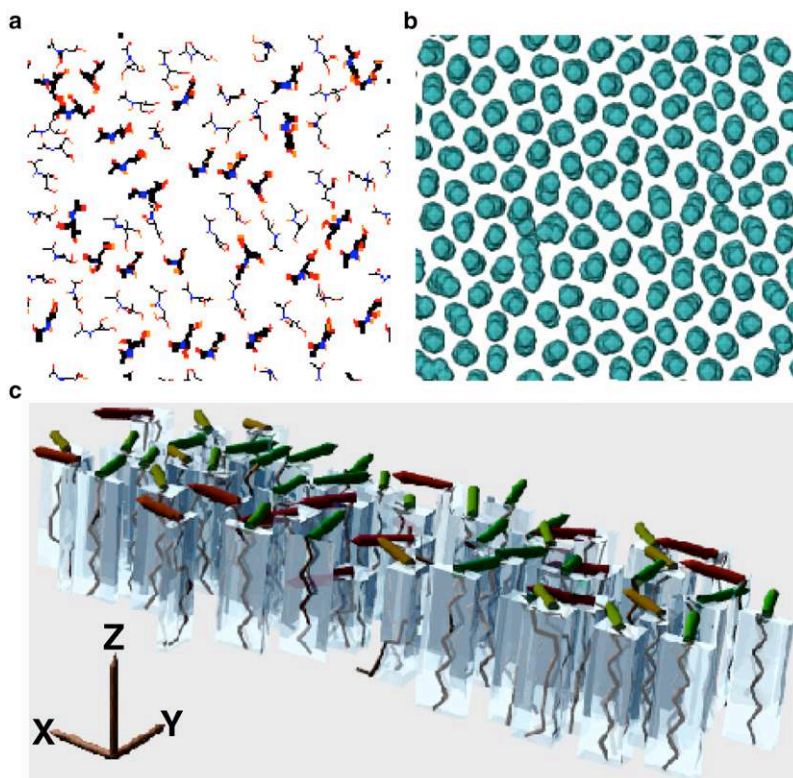
FIGURE 3 ( a ) Top view of CER molecule headgroup arrangement on one leaflet at T = 340 \text{ K} . The molecules are drawn in thick or thin lines, respectively, depending on whether the tangent of the angle between the line joining the end-atoms of the headgroup and the x axis is positive or negative. ( b ) Cross section of CER tail groups a few atoms below the headgroups, showing local hexatic order. ( c ) Side view of part of the lipid tails with (orthogonal distance regression) planes containing the tail atoms indicated by transparent boxes. The normals to these planes are indicated by solid rods on top of the boxes. In a crystalline configuration, the alignment of these planes is regular throughout the sample, while in the rotator phase, there are no correlations between the planes. In this case, local correlation between the hydrocarbon planes persists but allows slow rearrangement because the correlation is not perfect.
